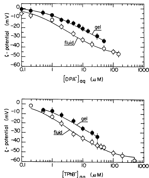
FIGURE 3 \zeta -potential isotherms of lipophilic ions and DPPC membranes. The isotherms for the gel state and the fluid state were obtained at 25 and 42°C, respectively. Conditions: pH 10, 0.03 M KCl, phosphate/citrate/borate buffer 0.002/0.002/0.0005 M; (a) DPA - , (b) TPhB - .
