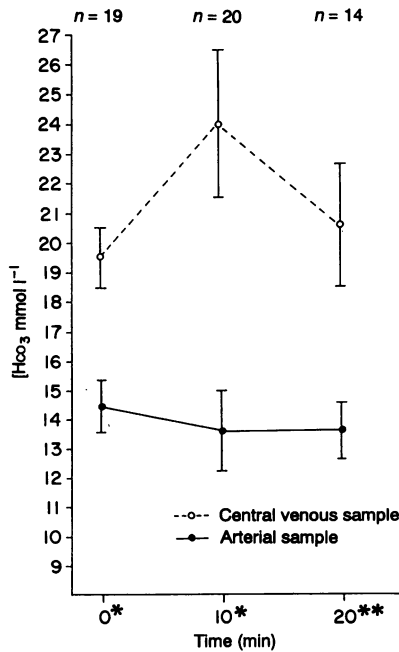
Fig. 3. Central venous and arterial calculated bicarbonate concentrations (mmol l -1 ). * P < 0.0001 , ** P < 0.01 .
