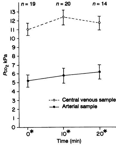
Fig. 2. Central venous and arterial P_{CO_2} (kPa). * P < 0.0001 .
