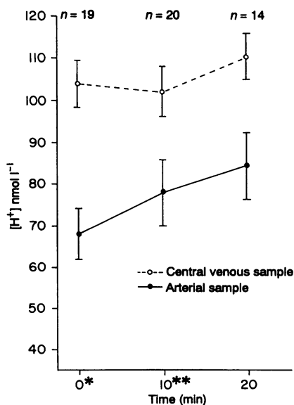
Fig. 1. Central venous and arterial H^+ concentrations (nmol l^{-1} ). * P < 0.0001 , ** P < 0.01 .
