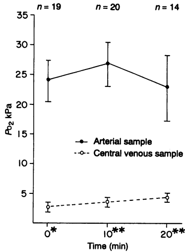
Fig. 4. Central venous and arterial P_{O_2} (kPa). * P < 0.0001 , ** P < 0.01 .
