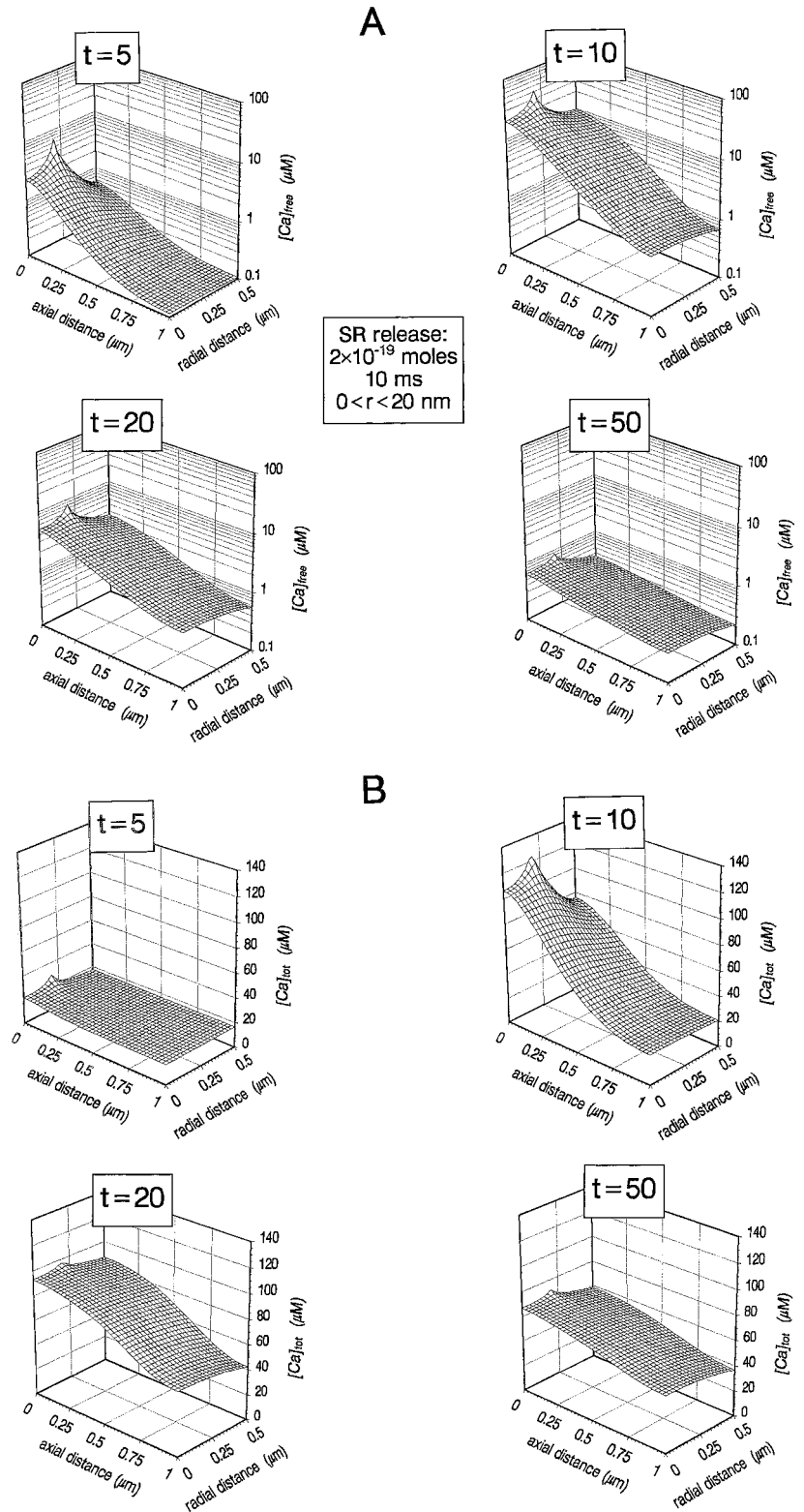
FIGURE 4 [Ca] for an SR release of 2 \times 10^{-19} moles. (A) Four snapshots of the free [Ca] in the sarcomere outside the cleft at t = 5, 10, 20, and 50 ms, as a function of radial and axial position in the shaded plane pictured in Fig. 1. Note that the portion of the curves at z = 0 from r = 0 to r = a = 200 nm are of [Ca] in the Z-line plane, outside the cleft, unlike the shaded portions of Figs. 2 A–C, which are of [Ca] inside the cleft (see text: Geometry of the Model). (B) The same as in A, but for total [Ca] (i.e., the sum of free Ca and Ca bound to troponin and calmodulin).
