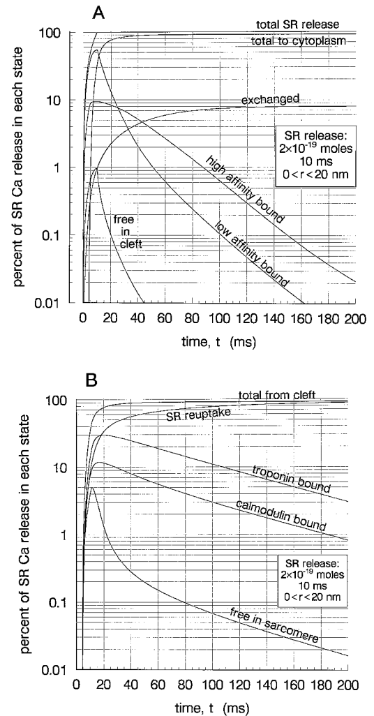
FIGURE 5 (A) The partition of Ca ions among the various possible states in or departed from the cleft: the fraction of the Ca ions released by the SR up to the time t that have left the cell via the Na-Ca exchanger, that have diffused radially out of the cleft and entered the sarcoplasm, or that are still within the cleft volume either free, or bound to low- or high-affinity sites. All amounts are normalized with respect to the total SR release and multiplied by 100%. Note that at t = 200 ms, 92% of the Ca has diffused to the general sarcoplasm and 8% has been transported out through the exchanger. (B) The fraction of Ca ions released from the SR up to the time t that are free in the sarcomere outside the cleft, that are bound to troponin or calmodulin, or that have diffused to the cylindrical boundary of the sarcoplasm, r = b = 500 nm, and have been taken up by the SR. At any instant the sum of the fractions equals the percentage of the total 10-ms-long SR release that has diffused out of the cleft up to that instant. Note that at t = 200 ms, ~3% of the Ca is bound to troponin, 1% is bound to calmodulin, 88% has been taken up by the SR, and 0.016% is free in the sarcoplasm. The remaining 8% has exited from the cell via the Na-Ca exchanger (see A).
