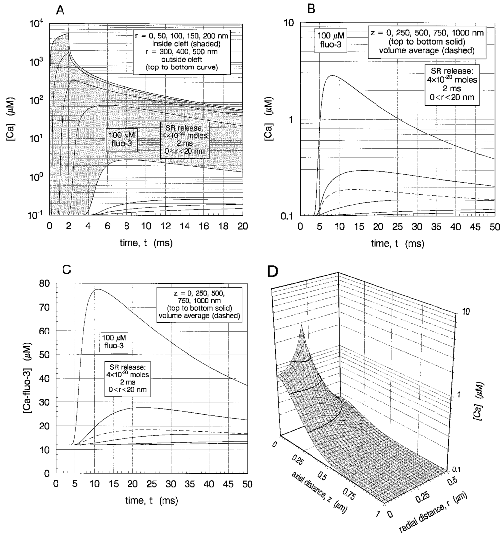
FIGURE 15 Same SR release of 4 \times 10^{-20} moles in a 2-ms-duration pulse, as in Fig. 14, but with the addition of 100 \mu\text{M} fluo-3 to the sarcoplasm. (A) [Ca] versus t at the eight radially spaced points in the z = 0 plane, shown in Fig. 1. (B) [Ca] versus t at the five axially spaced points at r = a = 200 nm, shown in Fig. 1. The dashed curves are the average of the [Ca] over the volume of the sarcomere outside the cleft. (C) Same as in B, but for [Ca-fluo-3] and volume average of [Ca-fluo-3]. (D) Snapshot at t = 8 ms, the instant of peak [Ca] outside the cleft, on the shaded plane in Fig. 1. The superimposed heavy curves are constant [Ca] contours. Comparing Figs. 14 A and B with 15 A and B, inside the cleft the effect of adding fluo-3 is negligible, but outside it is significant: the peak concentrations are lower and the peaks are delayed and broadened. Comparing Fig. 15 B ([Ca]) with Fig. 15 C ([Ca-fluo-3]) indicates an additional delay and broadening of the peaks for [Ca-fluo-3] transients compared to those for [Ca]. Comparing Figs. 15 D and 14 C indicates that the [Ca] transient is more localized spatially when 100 \mu\text{M} fluo-3 is present.
