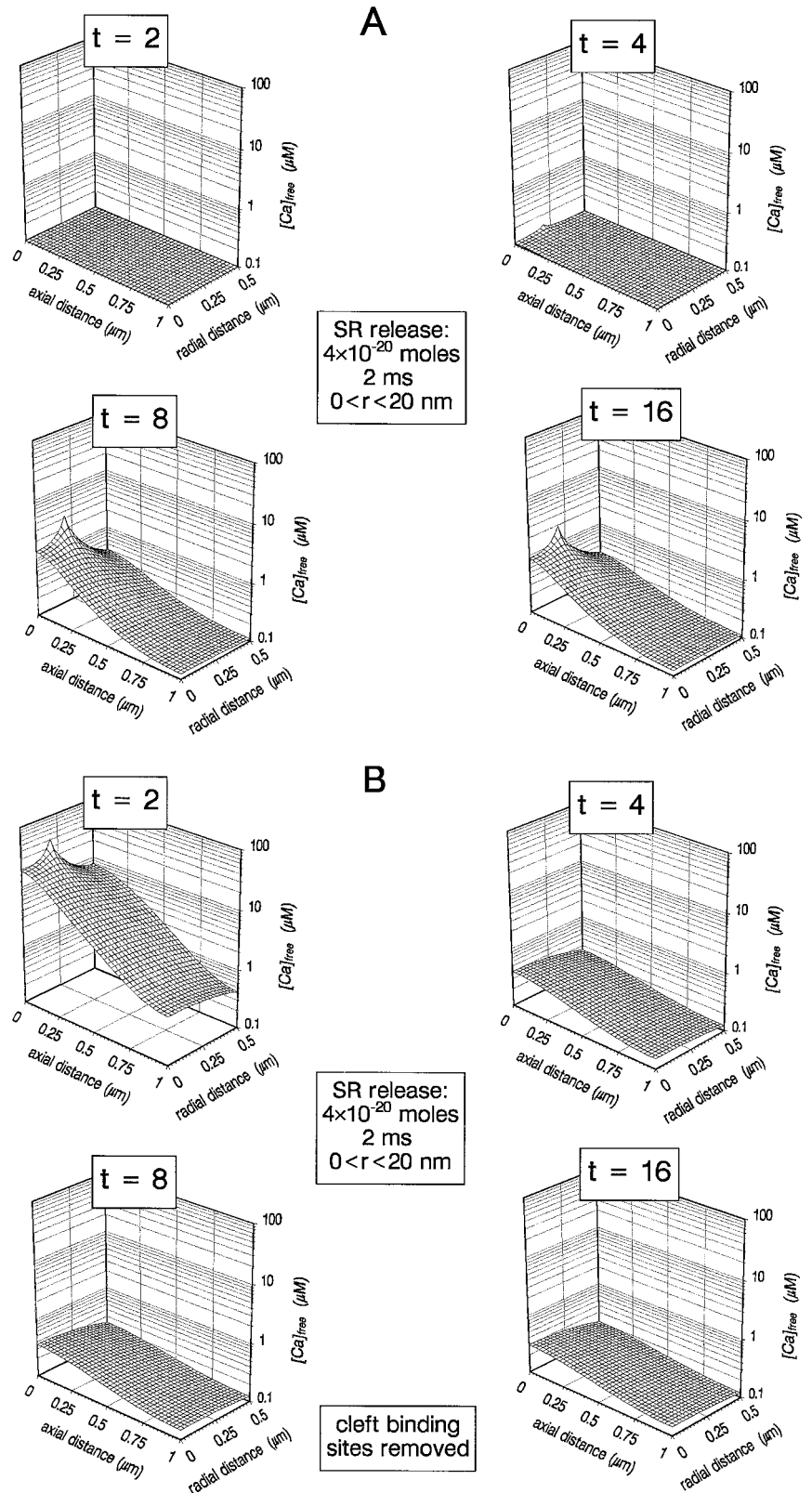
FIGURE 19 [Ca] snapshots at 2, 4, 8, and 16 ms for an SR release of 4 \times 10^{-20} moles in a 2-ms-duration pulse. (A) With and (B) without binding sites in the cleft. Note that at t = 4 ms, in A the response is just beginning to appear, whereas in B it has already decreased by two orders of magnitude from its peak.
