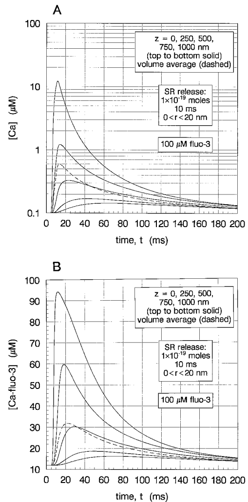
FIGURE 10 Same as in Fig. 8, but for an SR release of 1 \times 10^{-19} moles, with 100 \mu\text{M} fluo-3 added to the sarcoplasm. (A) [Ca] versus t at the five axially spaced points at r = a = 200 nm, shown in Fig. 1. The dashed curve is the average of the [Ca] over the volume of the sarcomere outside the cleft. Compare to Fig. 6 B for the same conditions without the added fluo-3. (B) Same as in A, but for [Ca-fluo-3] and volume average of [Ca-fluo-3].
