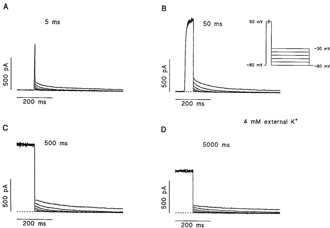
FIGURE 4 hKv1.5 currents after (A) 5-, (B) 50-, (C) 500-, and (D) 5000-ms pulses to +50 mV in 4 mM external K^+ (inset depicts pulse protocol). The amplitude of the current declined as the conditioning pulse duration was increased from 50 to 5000 ms, reflecting slow inactivation. However, the time course of deactivation was also modified with the apparent loss of the fast component of current decay after longer prepulses (compare B and D).
