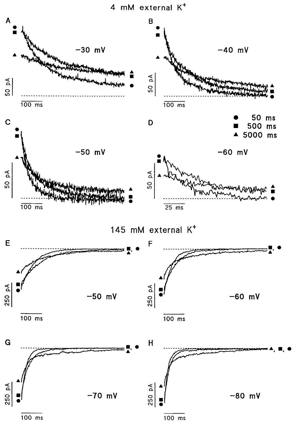
FIGURE 5 hKv1.5 tail currents after 50 (●), 500 (■), and 5000 ms (▲) at (A) -30 mV, (B) -40 mV, (C) -50 mV, and (D) -60 mV in 4 mM external K^+ and at (E) -50 mV, (F) -60 mV, (G) -70 mV, and (H) -80 mV in 145 mM external K^+ . A–D represent expanded and superimposed views of the tails currents from Fig. 4. Despite similar initial amplitudes after 50- and 500-ms prepulses, the decay is considerably slower after the 500-ms prepulse. After the 5000-ms prepulse, the initial amplitude was lower (due to partial inactivation), but the additional slowing resulted in a crossover phenomena (crossover was observed at each voltage in each experiment ( n \geq 4 )).
