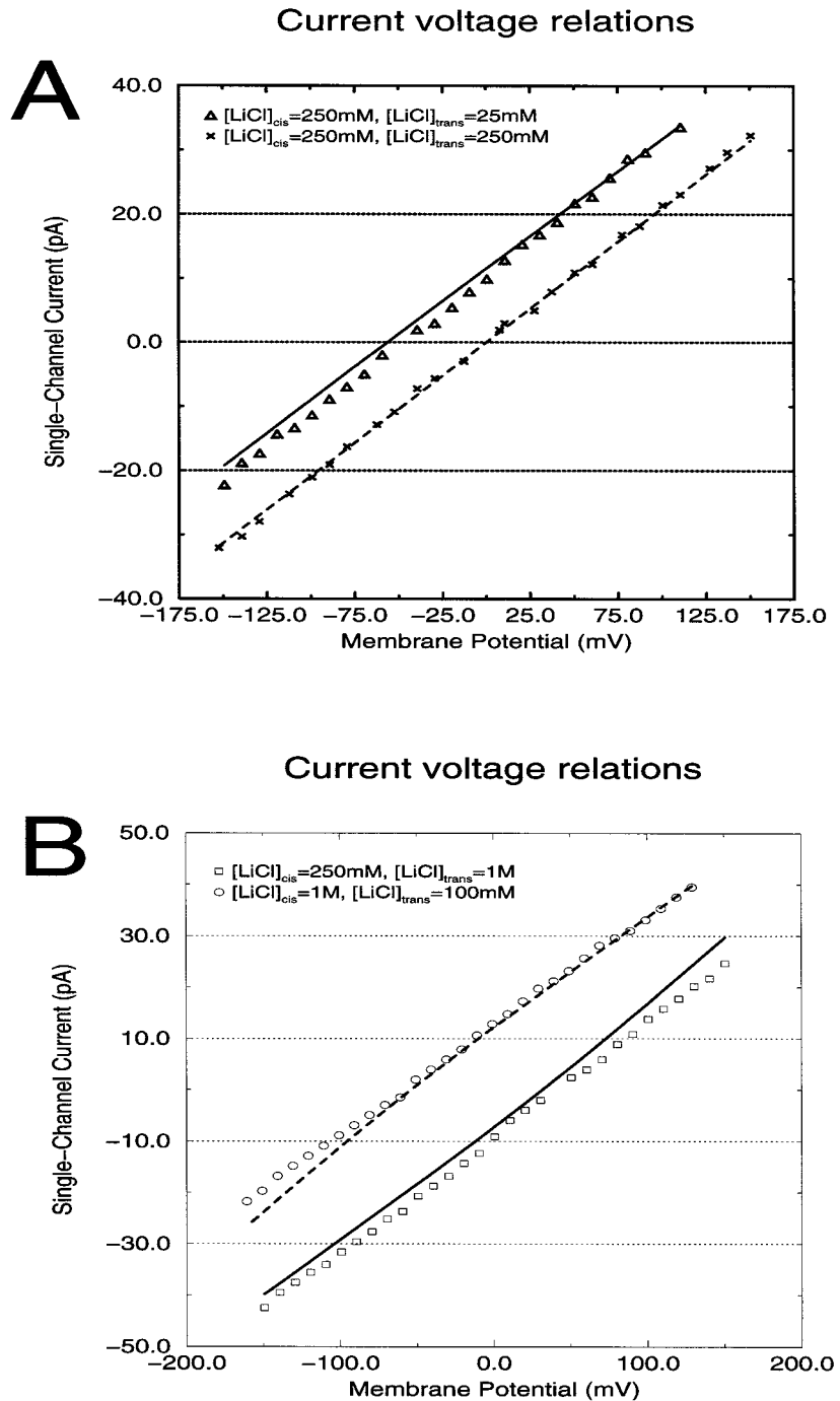
FIGURE 2 The current-voltage relations for LiCl are fitted simultaneously with I - V 's of NaCl, KCl, RbCl, and CsCl. The symbols show the experiment, and the lines are the fits of PNP. The salt solution is indicated in the legend next to the experimental symbols. There are four I - V 's for LiCl. We consider the lower panel poor fits, but they are later corrected in Fig. 11.
