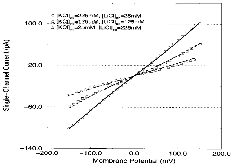
FIGURE 9 (A) The mole fraction plot of conductance of CRC of a mixture of KCl and LiCl at a total of 250 mM concentration. The filled circles are the experimental measurement of points of conductance. The dashed line is there just to connect the points. We have found a slight nonlinear mole fraction effect, but no anomalous mole fraction effect. (B) The predicted I - V 's for mixtures of lithium chloride and potassium chloride at a total ionic concentration of 250 mM. The three I - V 's shown here correspond to potassium mole fractions of 10%, 50%, and 90%. The points are the experimental dots, and lines are PNP predictions. The open circles are for 90% K, open squares are for 50% K, and open triangles are for 10% K. The I - V 's for pure LiCl are shown in Figs. 2 A, and 10. (C) The activities of lithium ions (90%) and potassium ions (10%) at a total of 250 mM along the CRC channel with and without the chemical binding of lithium ions. The part of the profiles in the baths is omitted. The occupancy of chloride ions is so low that it is omitted. The solid line is the profile of potassium ions, and the dashed line is the profile for lithium ions when there is no binding for lithium ions. Because symmetrical solutions are used in a typical mole fraction experiment, the corresponding concentration profiles are flat lines. Two flat lines will give a linear conductance versus mole fraction curve. The solid line with triangles is the profile of potassium ions, when there is a binding of lithium ions, and the dashed line with open circles is the profile of lithium ions. (Note that on the graph we have moved the binding region at 1–9 Å to show the effect clearly.) The curves show that the bound lithium ions repel the potassium ions, making a nonlinear mole fraction plot.
