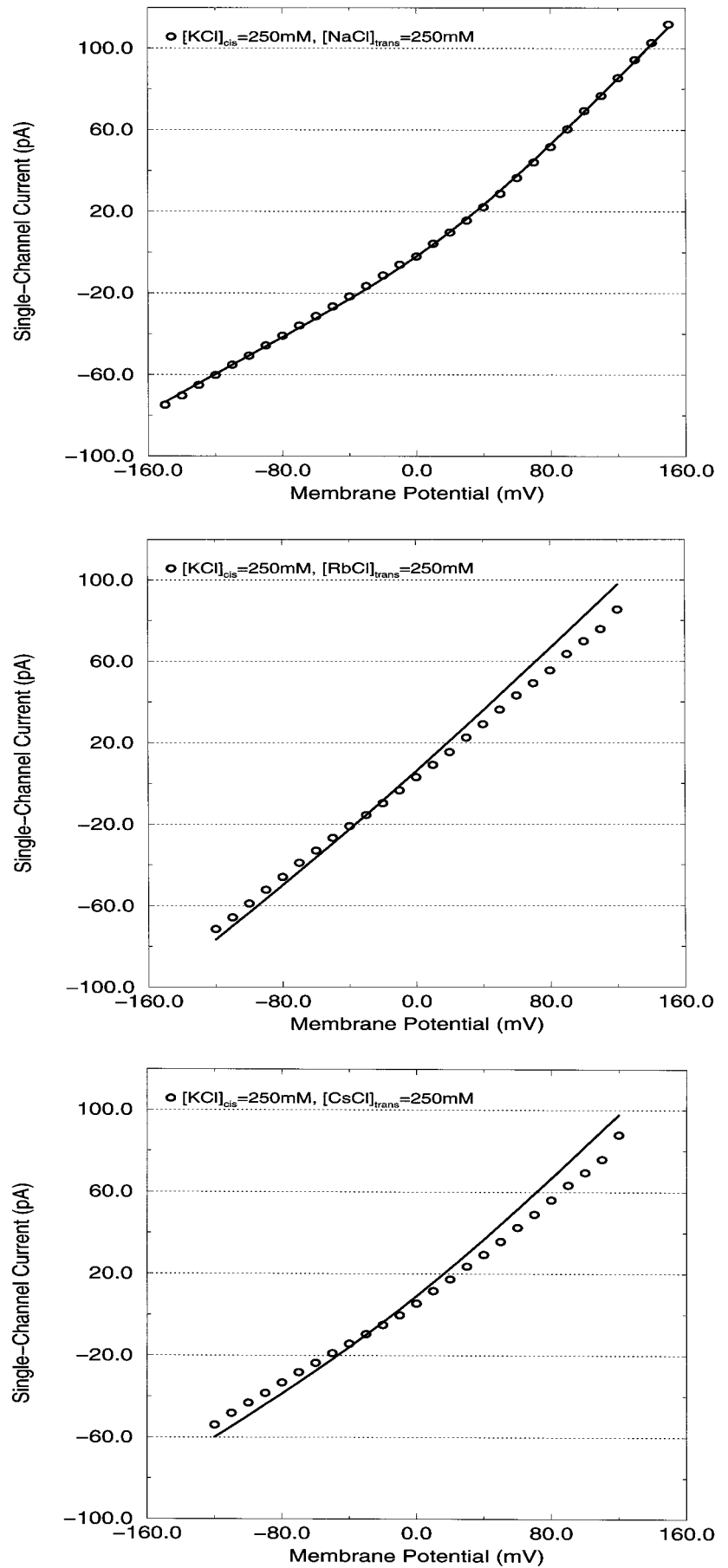
FIGURE 13 (A) The fit of the extended PNP to the measured current-voltage relation in the biionic condition of 250 mM KCl ( cis ) and 250 mM NaCl ( trans ) when \bar{\mu}(\text{Na}) = -25 mV. The open circles are the experimentally measured I-V points, and the solid line is the fit by the extended PNP. (B) The fit of the extended PNP to the measured current-voltage relation in the biionic condition of KCl ( cis ) and RbCl ( trans ) at 250 mM concentration when \bar{\mu}(\text{Rb}) = 0.9 mV. The convention is the same as the one used in A. (C) The fit of the extended PNP to the measured current-voltage relation in the biionic condition of 250 mM KCl ( cis ) and 250 mM CsCl ( trans ) when \bar{\mu}(\text{Cs}) = 1.2 mV. The convention is the same as the one used in A.
