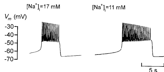
FIGURE 8 Computer simulations of the impact of changes in the intracellular Na + level ([Na + ] i ) on the β-cell bursting pattern. Bursts of action potentials in the presence of normal extracellular Na + and [Na + ] i were set to 17 mM (left). The reduction of intracellular Na + from 17 to 11 mM (right) led to a 60% increase in burst duration.
