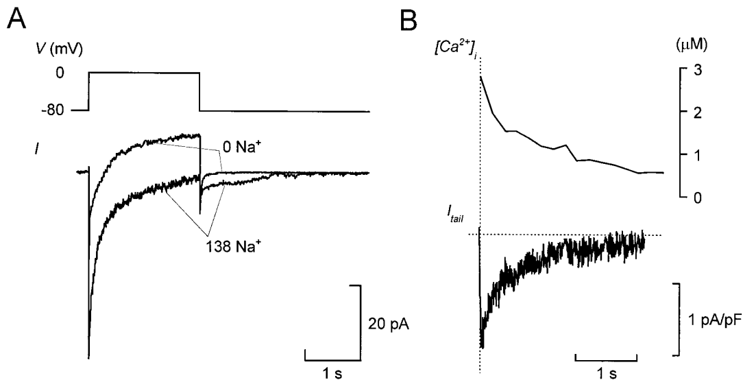
FIGURE 2 Whole-cell currents resulting from \text{Ca}^{2+} extrusion. (A) Whole-cell \text{Ca}^{2+} currents recorded in the perforated patch configuration in response to 2-s stimulations to 0 mV from a holding potential of -80 mV. Shown are the currents in the presence and absence of extracellular \text{Na}^+ (replacement by sucrose). Note the slow tail current (amplitude 3–4 pA) after the depolarization in the presence of \text{Na}^+ . (B) Time course of [\text{Ca}^{2+}]_i recovery and the \text{Na}^+ -dependent tail current. Traces represent the average data of six experiments in which \text{Na}^+ had been replaced by sucrose.
