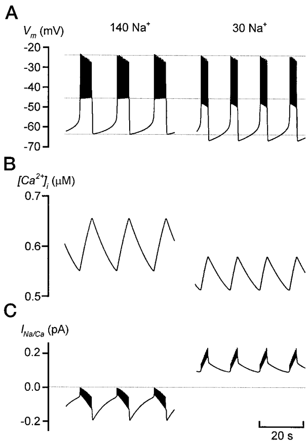
FIGURE 7 Computer simulations of electrical activity. (A) Influence of lowering extracellular Na + ([Na + ] o ) from 140 to 30 mM on simulated glucose-stimulated electrical activity. The model burst duration is reduced by 40% as a consequence of the changed [Na + ] o level. (B) Variations in model [Ca 2+ ] i levels in the presence of normal (left) and low extracellular Na + (right). (C) Corresponding currents carried by the Na/Ca exchange (I Na/Ca ) in the model cell. Observe that I Na/Ca during the burst changed from an inward depolarizing current in normal [Na + ] o to an outward current in low [Na + ] o .
