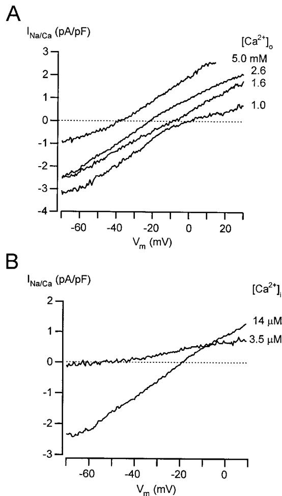
FIGURE 4 The influence of external and internal Ca^{2+} levels on the operation of the Na/Ca exchanger. (A) Net whole I-V relationships recorded at 1, 1.6, 2.6, and 5.0 mM extracellular Ca^{2+} . The traces shown are averages of 7 (1 mM), 7 (1.6 mM), 13 (2.6 mM), and 7 (5 mM Ca^{2+} ) cells. Extracellular Na^+ was replaced with choline ^+ to block the exchange current. (B) I-V curves recorded at 3.5 \mu M or 14 \mu M [Ca^{2+}]_i with an external Ca^{2+} concentration of 2.6 mM. The curves represent the averages of 13 (14 \mu M) and 8 (3.5 \mu M Ca^{2+} ) different cells.
