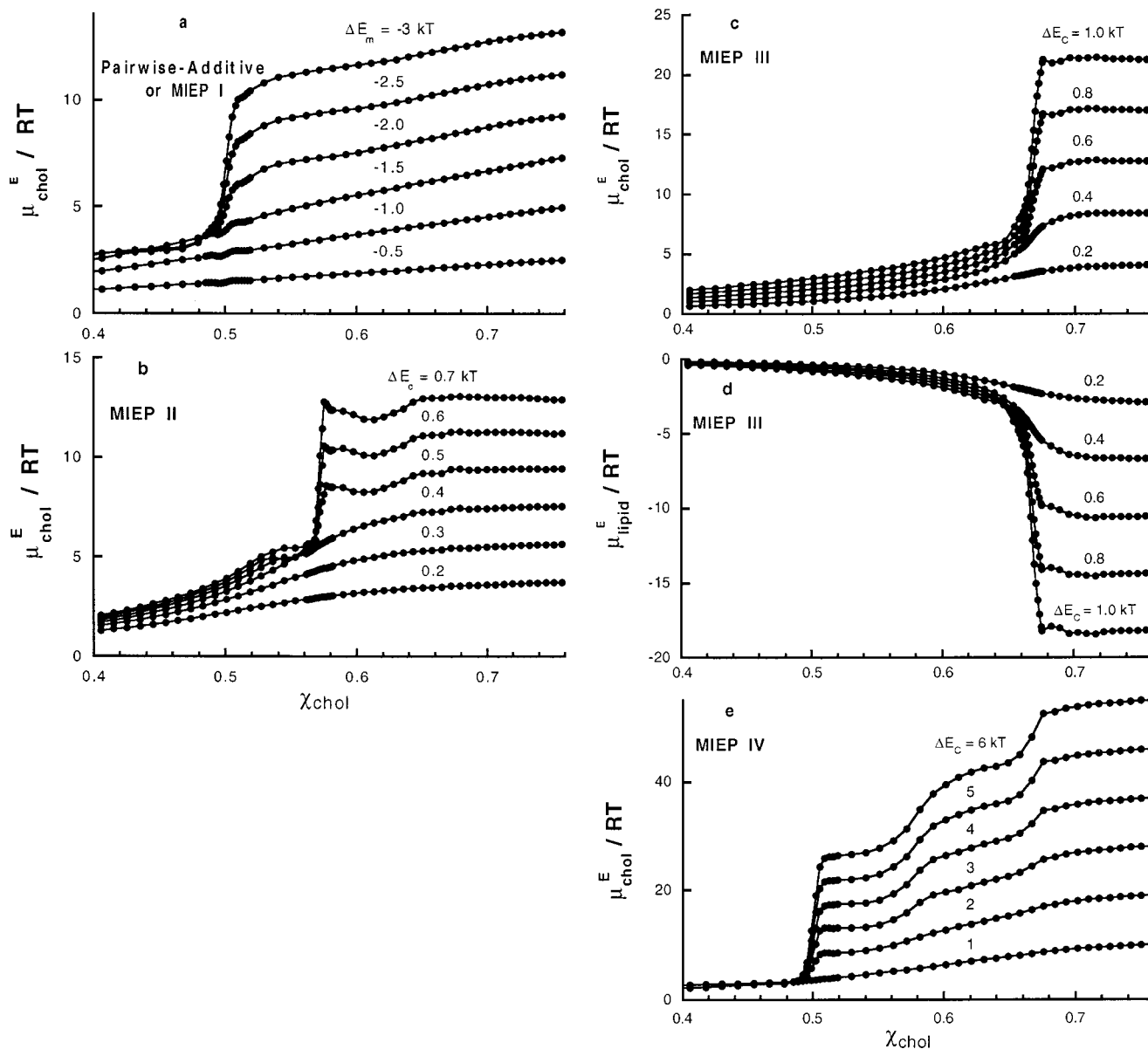
FIGURE 4 Excess chemical potential of cholesterol, \mu_{\text{chol}}^E , or of phospholipid, \mu_{\text{lipid}}^E , as a function of cholesterol mole fraction. (a) \mu_{\text{chol}}^E , simulated using pairwise-additive interactions, which is equivalent to MIEP I; (b) \mu_{\text{chol}}^E , simulated using MIEP II; (c) \mu_{\text{chol}}^E and (d) \mu_{\text{lipid}}^E , simulated using MIEP III; (e) \mu_{\text{chol}}^E , simulated using MIEP IV.
