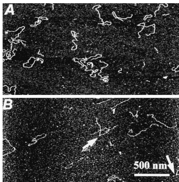
FIGURE 8 AFM images of linearized plasmid DNA deposited on AP-mica (A) and immobilized by photocross-linking to TO-mica (B). Several kinks in (B) are indicated with arrows. One of oriented molecules is marked with Fig. 1. The scan size for both images is 2.6 \mu\text{m} .
