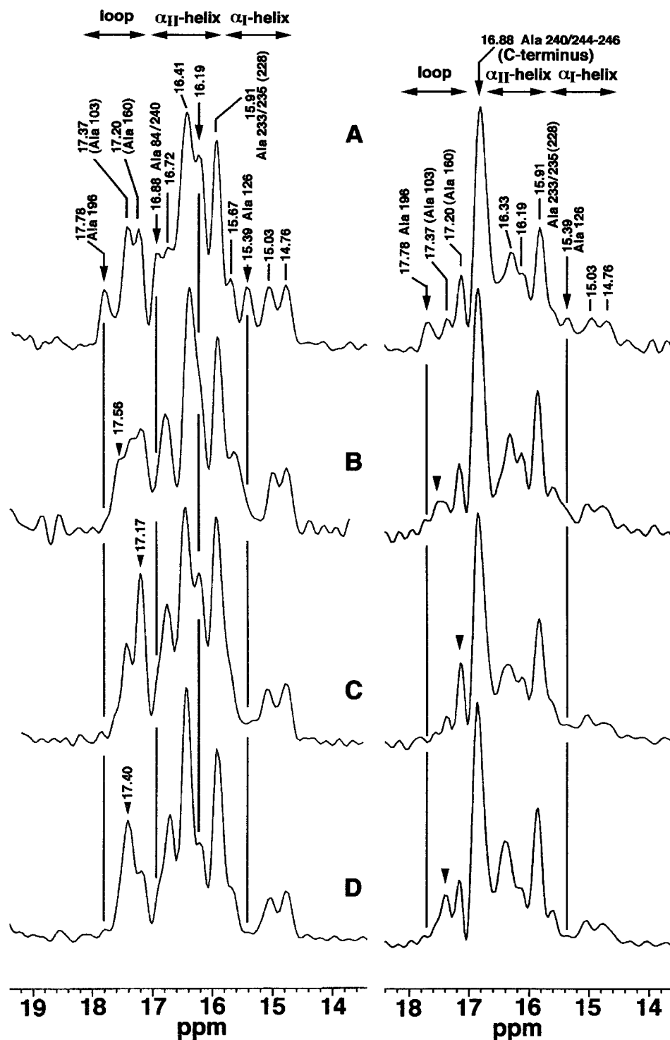
FIGURE 1 100.6 MHz ^{13}\text{C} CP-MAS (left) and DD-MAS (right) NMR spectra of [3-^{13}\text{C}] Ala-labeled wild-type bR (A), E194Q (B), E194D (C), and E204Q (D) at pH 7. Assigned signals for the wild type, so far completed, are given at the respective peaks, including tentative ones (parentheses), as discussed in this paper. The displaced peak positions for Ala ^{196} for a variety of the site-directed mutants are indicated by the wedges.
