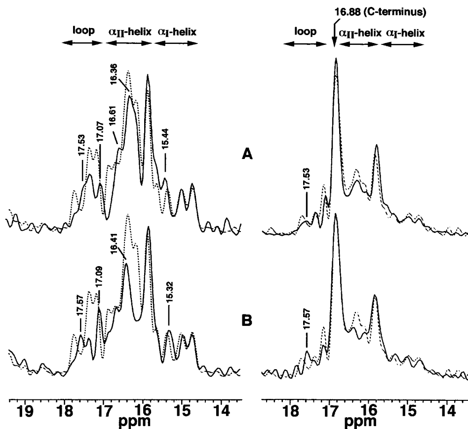
FIGURE 5 100.6 MHz ^{13}\text{C} CP-MAS (left) and DD-MAS (right) NMR spectra of [ 3\text{-}^{13}\text{C} ]Ala-labeled R82Q (A; pH 6) and R82Q/D85N (B; pH 7). The dotted spectra are for the wild type at pH 7, for comparison.
