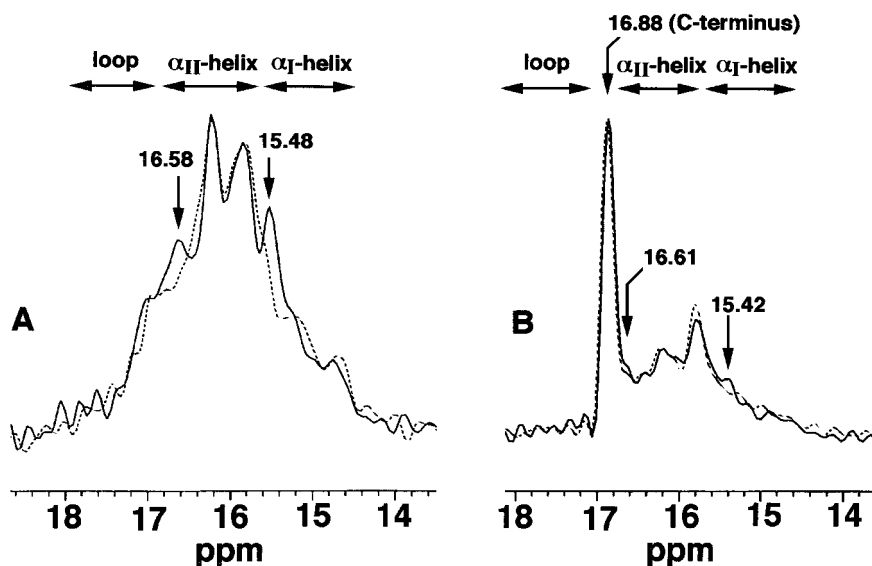
FIGURE 4 100.6 MHz ^{13}\text{C} CP-MAS (A) and DD-MAS (B) NMR spectra of [ 3\text{-}^{13}\text{C} ]Ala-labeled D85N (—) and wild type (.....) at pH 2.6 and 1.2, respectively.
