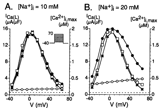
FIGURE 10 (A and B) Relationship between Ca^{2+} entry and Peak [Ca^{2+}]_i for two different concentrations of [Na^+]_i . (A) ( [Na^+]_i = 10 mM) and (B) ( [Na^+]_i = 20 mM) peak I_{Ca(L)} ( \times ; shown with reversed polarity) are shown together with three different [Ca^{2+}]_{i,max} curves. These [Ca^{2+}]_{i,max} curves are generated by three different modes of SR triggering: Ca^{2+} entering through any mechanism contributes to triggering SR Ca^{2+} release ( \bullet ), only Ca^{2+} carried by I_{Ca(L)} contributes ( \square ), and only Ca^{2+} carried by reverse-mode I_{NaCa} contributes ( \circ ). The dashed line indicates resting [Ca^{2+}]_i .
