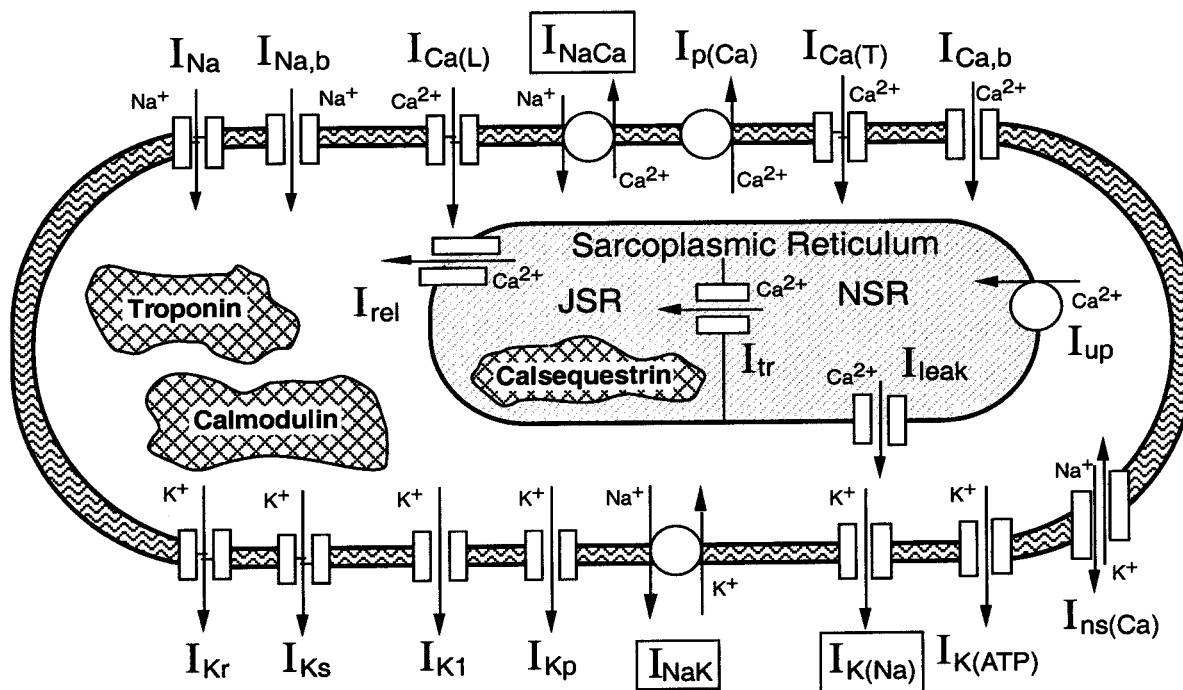
FIGURE 1 Schematic diagram of the dynamic Luo–Rudy (LRd) mammalian ventricular cell model. The major ion transporters, the sodium–potassium pump current, I_{NaK} and the sodium–calcium exchange current, I_{NaCa} , are highlighted, as well as the sodium-activated potassium current, I_{K(Na)} . Additional currents of significance in this study: I_{Na} , fast sodium current; I_{Ca(L)} , calcium current through L-type calcium channels; I_{Ca(T)} , calcium current through T-type calcium channels; I_{Kr} , fast component of the delayed rectifier potassium current; I_{Ks} , slow component of the delayed rectifier potassium current; I_{p(Ca)} , calcium pump in the sarcolemma; I_{Ca,b} , calcium background current; I_{up} , calcium uptake from the myoplasm to network sarcoplasmic reticulum (NSR); I_{rel} , calcium release from the junctional sarcoplasmic reticulum (JSR). For details see Luo and Rudy (1994a), Zeng et al. (1995), and Viswanathan et al. (1999). The LRd model code can be downloaded from the research section of http://www.CWRU.edu/med/CBRTC .
