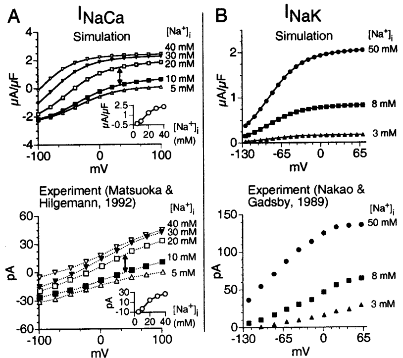
FIGURE 3 Current–voltage relationships for I_{NaCa} and I_{NaK} as a function of [Na^+]_i . (A) Simulated ( top ) and experimentally measured ( bottom , adapted from Matsuoka and Hilgemann, 1992) I_{NaCa} I - V relationships for 5 mM (△), 10 mM (■), 20 mM (□), 30 mM (▼), and 40 mM (▽) [Na^+]_i , obtained with 1 \mu M [Ca^{2+}]_i , 2 mM [Ca^{2+}]_o , and 150 mM [Na^+]_o . The insets show I_{NaCa} magnitude versus [Na^+]_i , measured at 20 mV, demonstrating saturation of the current with increasing [Na^+]_i . (B) Simulated ( top ) and experimentally measured ( bottom , adapted from Nakao and Gadsby, 1989) I_{NaK} I - V relationships for 3 mM (●), 8 mM (■), and 50 mM (▲) [Na^+]_i , obtained with 5.4 [K^+]_o , 140 [K^+]_i , and 145 mM [Na^+]_o .
