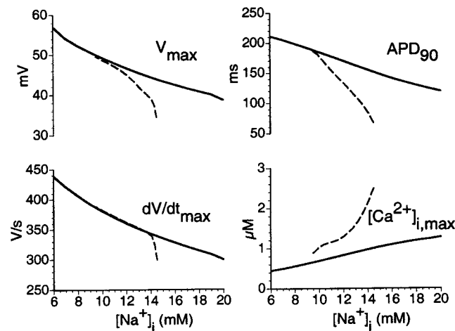
FIGURE 8 [Na^+]_i -dependent changes of action potential morphology and of peak [Ca^{2+}]_i . Changes in peak membrane voltage ( V_{max} ), action potential duration (APD), maximum rate of rise of the action potential upstroke ( dV/dt_{max} ), and peak calcium transient ( [Ca^{2+}]_{i,max} ) are shown for two different experimental protocols. The solid curves show the isolated effect of [Na^+]_i changes ( [Na^+]_i is clamped to an assigned value just before a single stimulus; same protocol as Fig. 7). The dashed curves show values computed after 5 min. of pacing at various cycle lengths, allowing all concentrations to vary (same protocol as in Fig. 5).
