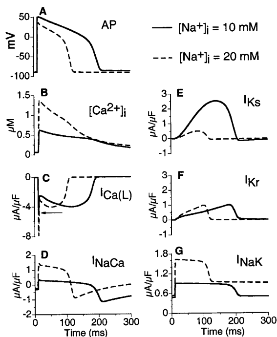
FIGURE 7 Isolated effect of elevated [Na^+]_i on the action potential. The figure shows the action potential (AP), calcium transient ( [Ca^{2+}]_i ), I_{Ca(L)} , I_{NaCa} , I_{Ks} , I_{Kr} , and I_{NaK} for two different concentrations of intracellular Na^+ , [Na^+]_i = 10 mM (solid lines) and [Na^+]_i = 20 mM (dashed lines). For the curve of I_{Ca(L)} (Panel C), the arrow indicates the peak of the current for [Na^+]_i = 10 mM.
