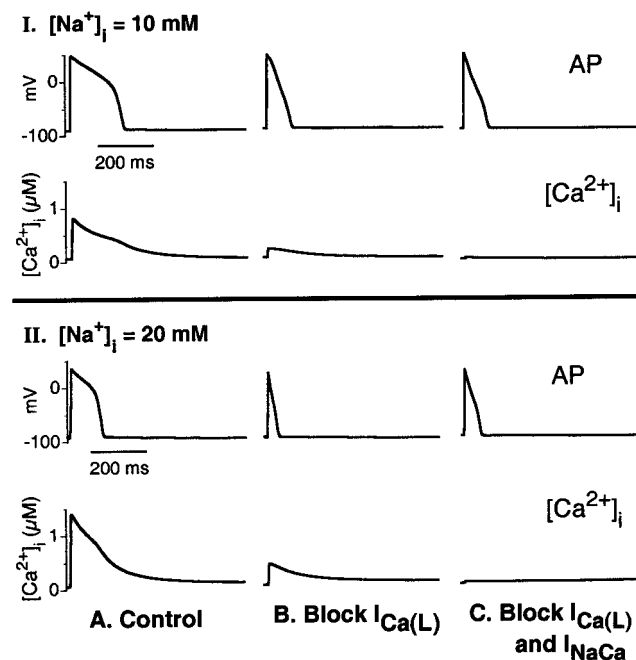
FIGURE 11 Contribution of I_{Ca(L)} and I_{NaCa} to Ca^{2+} release during the action potential. Action potentials and their corresponding Ca^{2+} transients are shown for (A) control conditions, (B) conditions of I_{Ca(L)} block, and (C) both I_{Ca(L)} and I_{NaCa} block. Channel block is applied just before stimulus, ensuring equal SR loading. Panel I shows results for physiologic [Na^+]_i = 10 mM. Panel II shows results for elevated [Na^+]_i = 20 mM (sodium overload).
