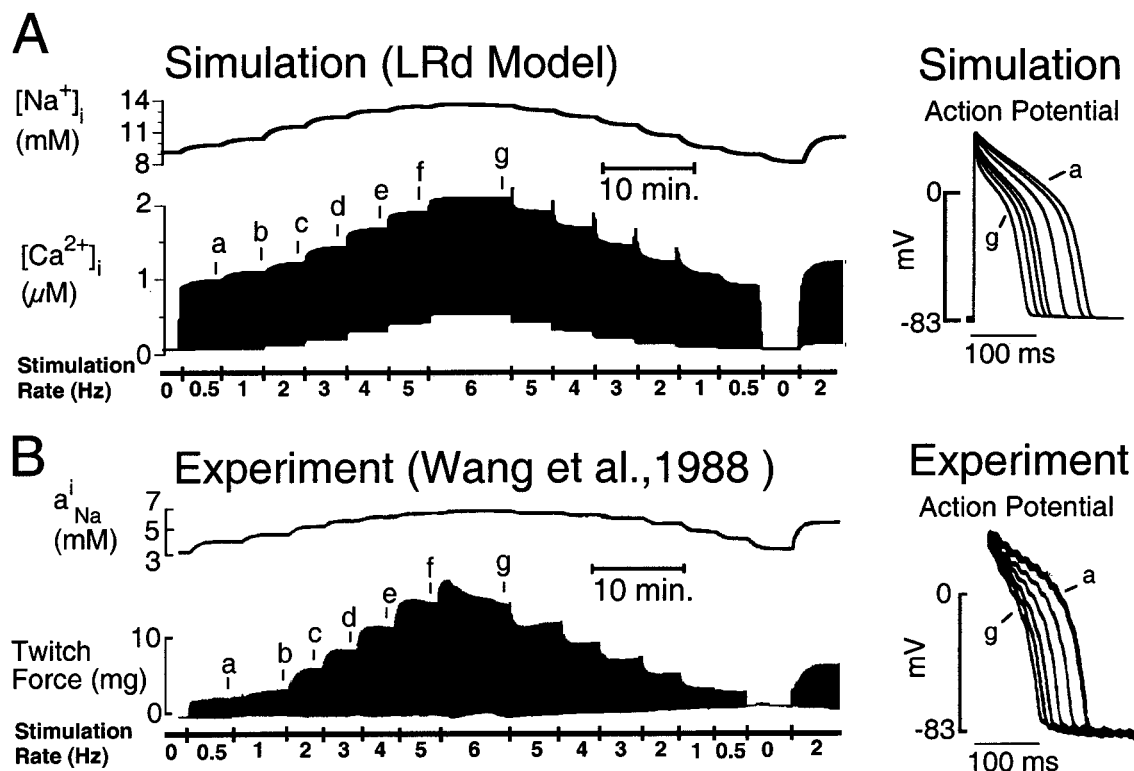
FIGURE 4 [Na^+]_i and [Ca^{2+}]_i as a function of pacing frequency. (A) Simulated concentration-frequency staircase, showing changes of [Na^+]_i and [Ca^{2+}]_i during a staircase protocol where frequency is stepped from 0.5 to 1 Hz and then to 6 Hz in increments of 1 Hz (5 min. at each pacing frequency). After 10 min. of pacing at 6 Hz, frequency is stepped down in reverse order. (B) The corresponding experiment showing measured intracellular sodium activity ( a_{Na}^i ) and twitch force for the same protocol (Wang et al., 1988). Both simulation and experiment were conducted using 5.4 mM [K^+]_o , 1.8 mM [Ca^{2+}]_o , and 137 mM [Na^+]_o . To the right of (A) and (B), the corresponding computed and measured action potentials at times a–g are shown.
