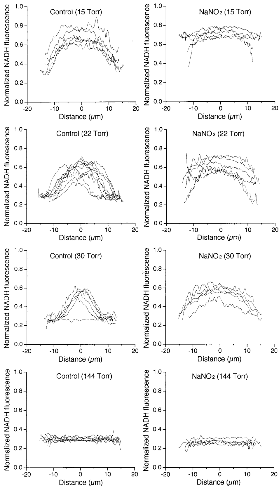
FIGURE 3 Radial profiles of the NADH fluorescence intensity for individual cardiomyocytes. Superfusion gas O_2 concentrations were 20.2% (144 Torr), 4.08% (30 Torr), 3.14% (22 Torr), and 2.09% (15 Torr). Distance = 0 corresponds to the center of the cell. Data from cells in which the width was >32 \mu\text{m} or <24 \mu\text{m} were not included. Cellular respiration was stimulated by 1 \mu\text{M} CCCP. Photobleaching was not compensated for.
