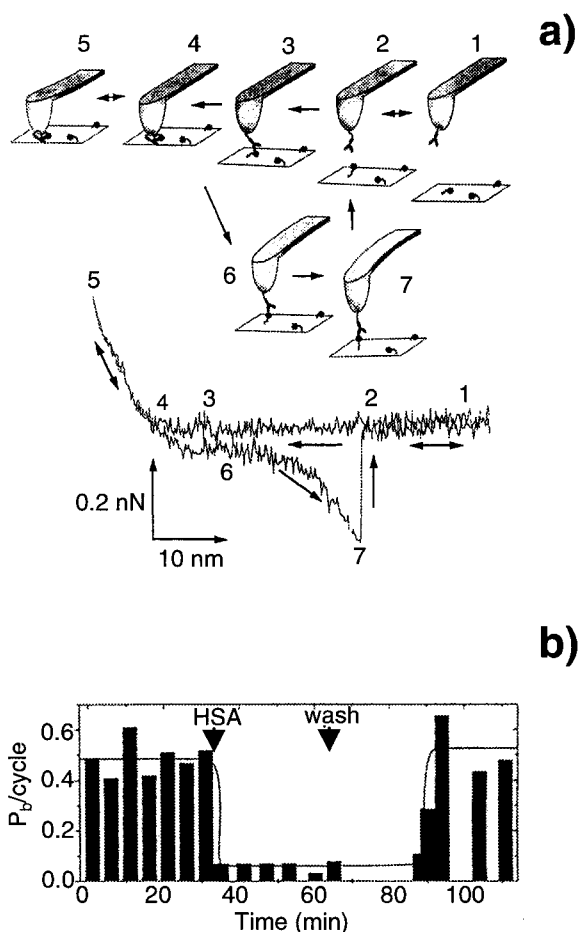
FIGURE 3 (a) Force-distance curve generated by Hinterdorfer and co-workers (1996). Both antibody and antigen are covalently bound to the tip and surface, respectively, via a bifunctional PEG spacer. During the approach of the tip to the surface, the line 1–5 is followed. During the retraction of the tip from the surface, the tip follows the line 6–7, indicating a delayed rupture that is attributed to the involvement of the spacer in the interaction. (b) Binding probability of antibody on the tip as a function of time. As indicated by the arrows, the addition of excess antigen to solution causes the binding probability to drop almost to zero. It recovers \sim 25 min after washing with buffer. Panels (a) and (b) are reprinted by permission from Hinterdorfer and co-workers ( Proc. Natl. Acad. Sci. USA , 93:3477–3481, © 1996, National Academy of Sciences).
