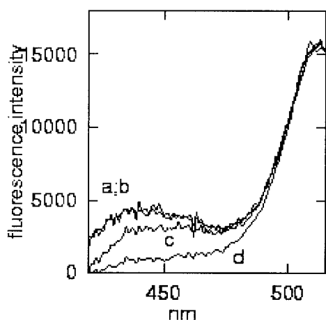
FIGURE 1 Fluorescence emission spectra of the pyranine-lac permease complex. The emission spectra were measured with excitation at \lambda = 350 nm with a solution containing 5 \mu\text{M} lac permease, 0.018\% LM, 100 \mu\text{M} HEPES buffer, \text{pH} = 6.5 . Traces a and b were recorded in the presence of 80 \text{ nM} pyranine or 80 \text{ nM} pyranine plus 20 \text{ mM} sucrose. Trace c was recorded after addition of 20 \text{ mM} TDG. Trace d was measured after addition of NaCl to final concentration of 50 \text{ mM} and is identical with the spectrum recorded with 80 \text{ nM} pyranine in LM.
