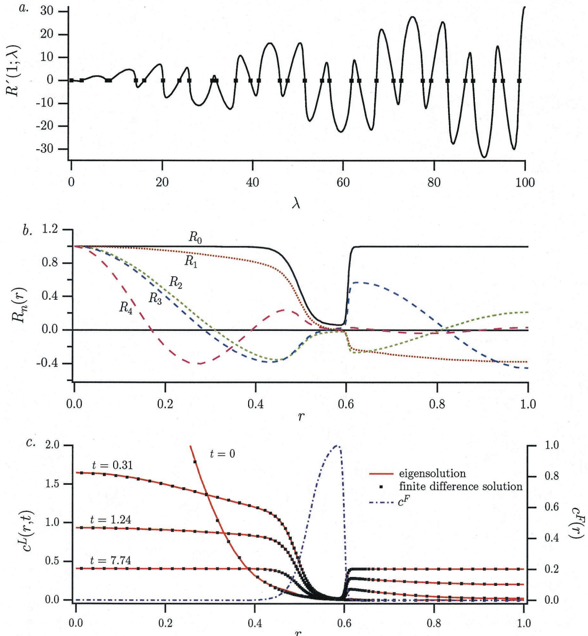
FIGURE 4 (a) Graphical representation of R'(1; \lambda) , corresponding to the left-hand side of the characteristic equation associated with the eigenvalue problem. As \lambda varies, so does R'(1; \lambda) . The eigenvalues, corresponding to the roots of the characteristic equation (dots), occur where R'(1; \lambda) vanishes. (b) The first five eigenfunctions, R_n(r) . To within a constant multiplicative factor, the eigenfunction, R_0(r) , corresponds to the equilibrium distribution of c^L . (c) Comparison of the solutions obtained by the finite-difference method versus the eigenfunction expansion (truncated after the first 15 terms); c^F is also shown. For all panels, F = 4744 , B = 4000 , Q = 200871 , m = 5 , r_g = 0.52 , \Delta r_g = 0.2 , r_{ec} = 0.6 , and \Delta r_{ec} = 0.03 .
