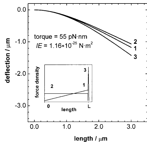
FIGURE 1 Static deformation of an elastic cantilever under three types of load distributions over its length (see inset). (1) Linearly increasing load as caused by a viscous drag on a rotating filament in a homogeneous fluid. (2) Uniformly distributed load (idealized friction at a solid surface). (3) Concentrated force acting on the very end of the cantilever (obstacle at the surface).
