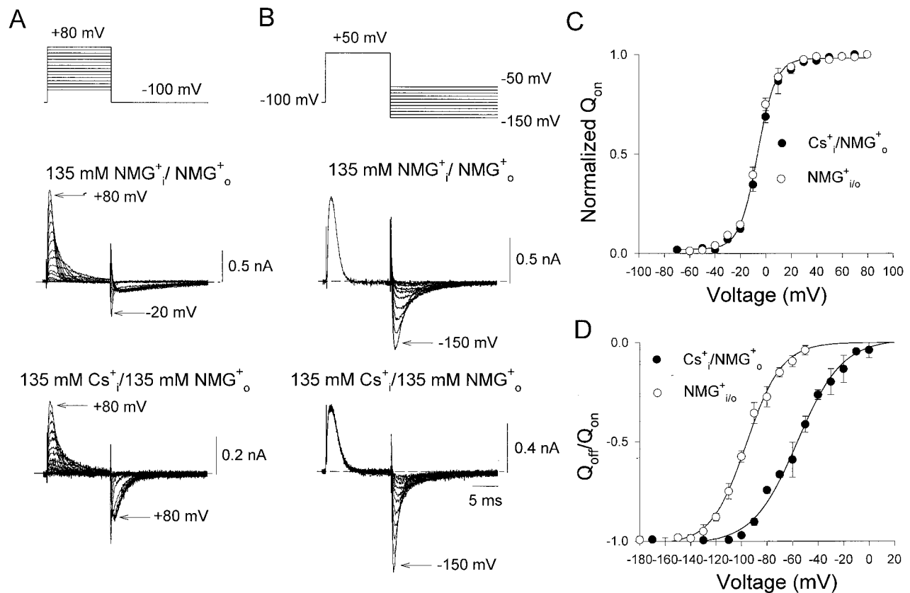
FIGURE 1 Gating charge immobilization on repolarization in the Kv1.5 NCM is caused by a rapid shift in the voltage dependence of charge return. (A) Off-gating currents after 12-ms depolarizations from -60 to +80 mV. Voltage protocol is shown at the top. Currents in the middle panel were recorded with symmetrical NMG + i /NMG + o solutions. Currents in the lower panel were recorded with 135 mM Cs + i substituted for the NMG + i . (B) Currents in the middle and lower panels were recorded on repolarization to a range of potentials between -50 and -150 mV, after a step depolarization to +50 mV, as illustrated by the protocol in the top panel, and under the same ionic conditions as in A. (C) Voltage dependence of Q_{on} for the experiments shown in A. The V_{1/2} for the fitted curve was -6.3 \pm 0.4 mV, with a slope factor k of 7.3 \pm 0.3 mV ( n = 20 ). (D) Voltage dependence of Q_{off}/Q_{on} for the experiments shown in (B), for NMG + i /NMG + o (○) and Cs + i /NMG + o (●). For NMG + i /NMG + o , the V_{1/2} was -96 \pm 0.6 mV; k was 14 \pm 0.6 mV ( n = 8 ). For Cs + i /NMG + o , the V_{1/2} was -56 \pm 1.3 mV and k was 17 \pm 1.2 mV ( n = 8 ).
