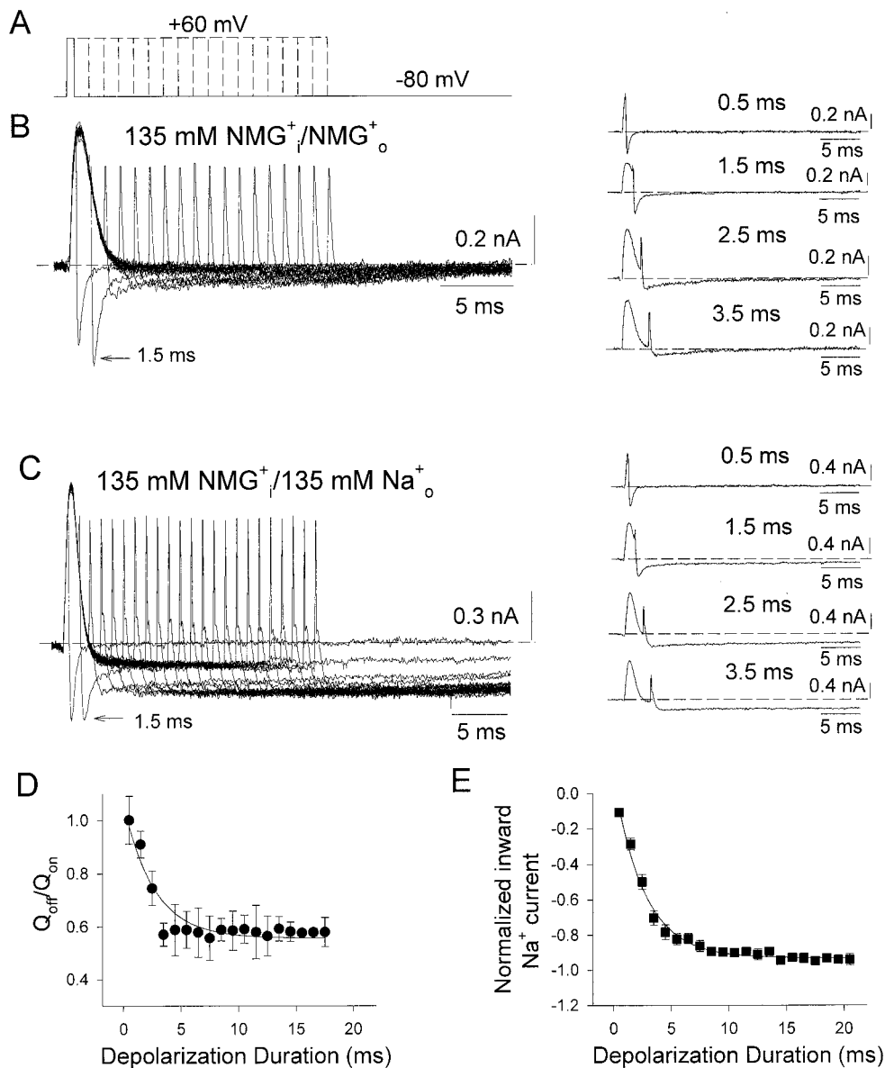
FIGURE 5 The time dependence of Q_{\text{off}} immobilization matches the time dependence of Na + current appearance through the NCM. (A) The pulse protocol used to collect data in B and C. (B) On- and off-gating currents from -80 to +60 mV, in response to increasing pulse duration. The initial duration was 0.5 ms and this was incremented by 1 ms for each cycle. The pulses were applied at 0.2 Hz. Envelopes of gating current were obtained with symmetrical NMG + (B), or with 135 mM Na + o (C). The right panels in each case illustrate selected on- and off-gating currents at increasing pulse durations as indicated. Note that the slowing of off-gating current return matches the increase in sustained inward Na + current (B, C, right). (D, E) Timecourse of charge immobilization ( Q_{\text{off}}/Q_{\text{on}} ) and inward Na + tail development with pulse duration. Charge immobilization was measured as the off-/on-gating charge at each pulse duration. The Na + current was measured at the peak inward current level. In each case data were from 9 cells, and for E, decay was fit with a single exponential ( \tau = 2.7 \pm 0.2 ms), shown as a line through datapoints. The same fit was applied to data in D.
