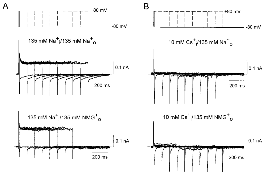
FIGURE 7 Effects of 135 mM Na i + or 10 mM Cs i + on Na + tail currents in NCM channels. (A) Pulse protocol is shown at the top, with an initial 10-ms depolarization and 100-ms increments. The pulses were applied at 0.2 Hz. Middle , membrane currents obtained using top panel protocol with symmetrical 135 mM Na + as indicated. Bottom , the same experiment as in the middle but with NMG o + to show the disappearance of Na + tail currents. Data in the middle and bottom were obtained from the same cell. (B) Pulse protocol as in A ( top ). Middle , experiment carried out on NCM channels with 10 mM Cs i + and 135 mM Na o + . Data show that with 10 mM Cs i + , the Na + tail currents were prevented, which is supported by the control experiment at the bottom with 10 mM Cs i + /135 mM NMG o + . Data shown at the middle and bottom were obtained from the same cell.
