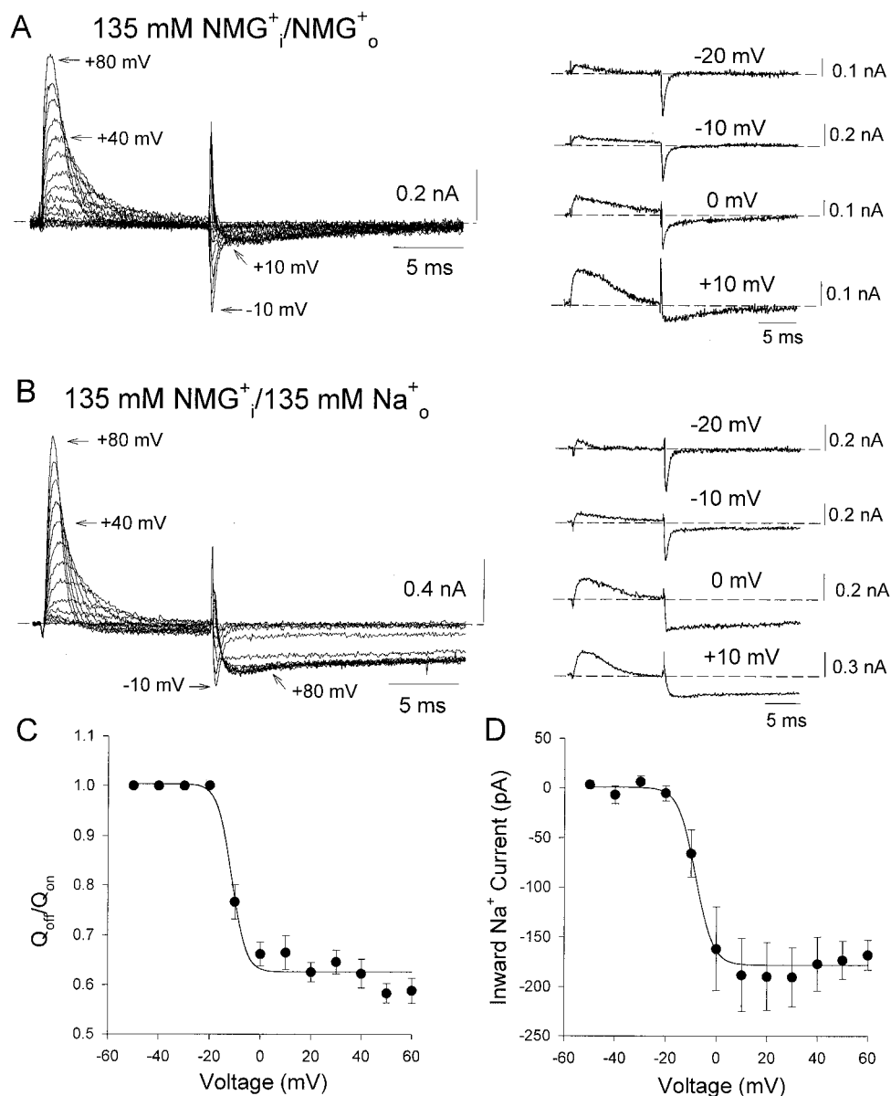
FIGURE 4 The voltage dependence of Q_{\text{off}} immobilization matches that of Na + currents through the NCM. ( A , B ) Gating current-voltage relationships induced by depolarizations from -100 mV to between -60 mV to +80 mV in 10 mV steps, with symmetrical NMG + ( A ), or with 135 mM Na + ( B ). The right panels in each case illustrate selected pulse potentials between -20 and +10 mV. Note that in all cases, repolarization potential was -100 mV. ( C ) Voltage dependence of charge immobilization measured as Q_{\text{off}}/Q_{\text{on}} as a function of potential, matches the voltage dependence of inward Na + current ( D ), measured as the sustained current level at the end of repolarization. For NMG + i /Na + o the V_{1/2} for sustained Na + current was -12.2 \pm 0.9 mV and k was 3.4 \pm 0.9 mV ( n = 6 ). For NMG + i /NMG + o the V_{1/2} for off-gating charge immobilization was -11.3 \pm 1.1 mV and k was 2.8 \pm 1.5 mV ( n = 7 ).
