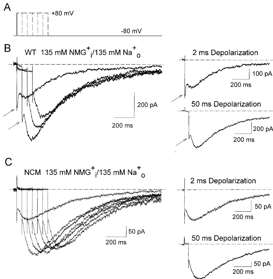
FIGURE 3 Both WT and NCM channels rapidly enter the inactivated state in the absence of internal univalent metal cations. (A) The pulse protocol used to collect data in B and C. Cells were pulsed from -80 mV to +80 mV for durations from 2 ms increasing to 50 ms for the second depolarization, and subsequently incrementing 50 ms each cycle. Pulses were given at a cycle interval of 20 s. (B, C) WT and NCM current data, respectively, obtained using the protocol described in A. Tracings for separate depolarizations have been superimposed in the left panels and those for 2-ms and 50-ms depolarizations are shown separately in the right panels. Note the absence of an initial inward tail transient in NCM channels after short depolarizations (arrow on WT data).
