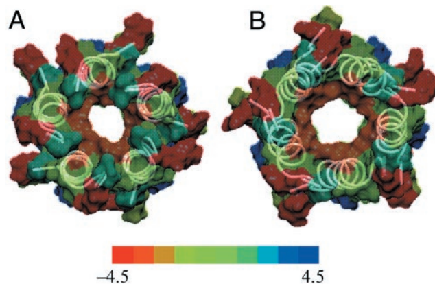
FIGURE 6 Homopentameric TM2 pore architectures (C-terminal views) of human \alpha_1 GlyR after extensive energy minimization in a fully hydrated DMPC membrane: (A) the helical axes are parallel to the pore axis, and (B) helical axes are tilted by 10^\circ relative to the pore axis. Notice the difference in pore diameter. The residues are colored in the same hydrophobic scale as in Fig. 4. The hydrophilic orange rings in the pore are composed of side chains of Q14', which might play an important role in channel gating (see Discussion). Online supplementary information: An animation is provided to offer a pictorial view of NMR-derived pore architecture (C-terminal views, after extensive energy minimization in a fully hydrated DMPC membrane) and the proposed gating model by the entire TM2 tilting movement. The side chains of Q266 form the top orange ring within the pore.
