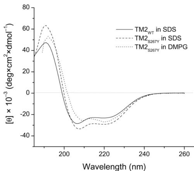
FIGURE 1 CD spectra of the functional segments of the pore-lining second transmembrane domain (TM2 WT ) of human glycine receptor \alpha_1 subunits in SDS micelles (solid line) and the anesthetic-insensitive TM2 S267Y mutant in SDS micelles (dashed line), and in DMPG lipid bilayers (dotted line). Spectra of the same peptides in DPC are very similar. The fraction of \alpha -helical conformation for TM2 WT and TM2 S267Y in micelles can be estimated based on the mean residue molar ellipticity at 222 nm to be 70% and 91%, respectively. All spectra were averages of three scans recorded at 30°C after subtraction of the reference spectra of the media.
