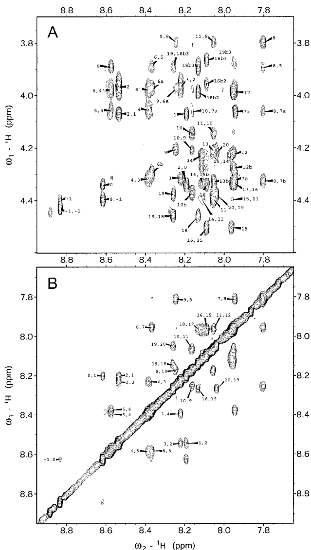
FIGURE 3 Representative 750-MHz 1 H-NOESY spectrum of GlyR TM2 in DPC micelles, showing (A) the H N -H α (fingerprint), and (B) the H N -H N regions. The exceptional resolution at high magnetic field allows for complete sequence-specific assignments and structural determination. All assigned peaks are labeled using the relative numbering system of the peptide sequence and following the ω 2 , ω 1 convention.
