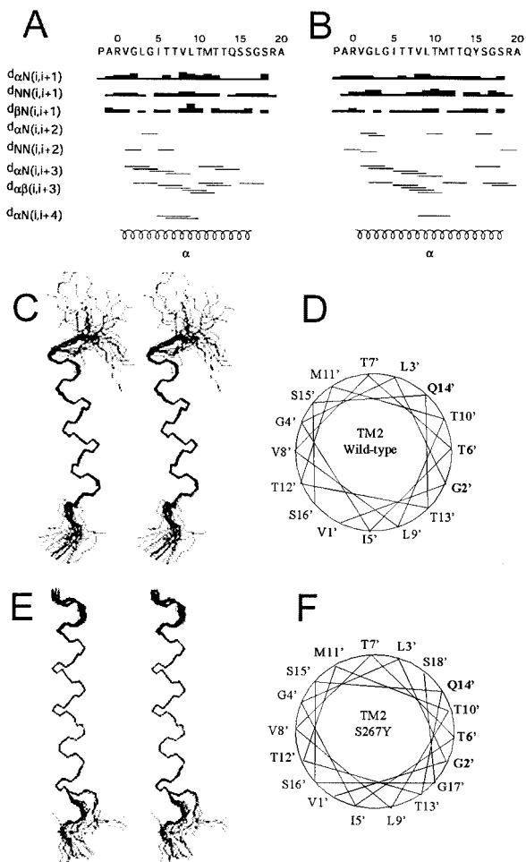
FIGURE 4 NMR determination of the TM2 structures of human glycine receptor. Sequential and mid-range NOE connectivity is plotted for the functional α 1 GlyR TM2 WT (A) and its anesthetic-insensitive TM2 S267Y mutant (B). Lines indicate that the NOEs were unambiguously identified and assigned; the widths of the lines are related to the observed NOE intensities. An α-helical pattern can be identified from V1' to S16' in TM2 WT and from V1' to S18' in TM2 S267Y . The first 30 lowest energy structures (stereo view, C-terminals at top) are depicted for TM2 WT (C) and TM2 S267Y (E) in SDS micelles. Structures in DPC are very similar. The corresponding helical wheels (D and F) revealed a well-defined hydrophilic face along the helix, composed of G2', L3', T6', T7', T10', Q14', G17', and S18', which either line or border the channel pore.
