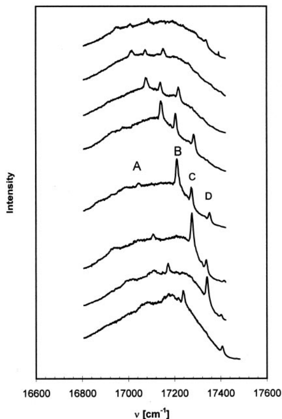
FIGURE 1 The FLN spectra of MgMP/DMSO (7 mM) measured at 10 K and ambient pressure. Excitations (from bottom to top ): 551 nm (18,148 \text{cm}^{-1} ), 553, 555, 557, 559, 561, 563, 565 nm (17,700 \text{cm}^{-1} ). The lines A, B, C, and D belong to the 896, 730, 669, 592 \text{cm}^{-1} vibrations of the excited state.
