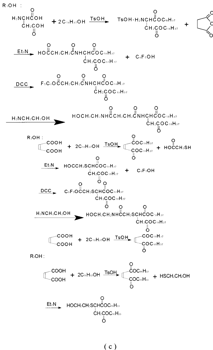
FIGURE 1 The molecular structures of the synthetic lipids and the scheme of the preparation process. (a) The structures of the three kinds of synthetic lipids. (b) The scheme of the preparation process, where ROH is the tail-connector-spacer alcohol (TSCOH) of the synthetic lipids. (c) Synthesis of the tail-connector-spacer alcohol (TSCOH), where R_1OH , R_2OH , and R_3OH represent TSCOH of DS8PC, DS6PC, and DS3PC, respectively.
