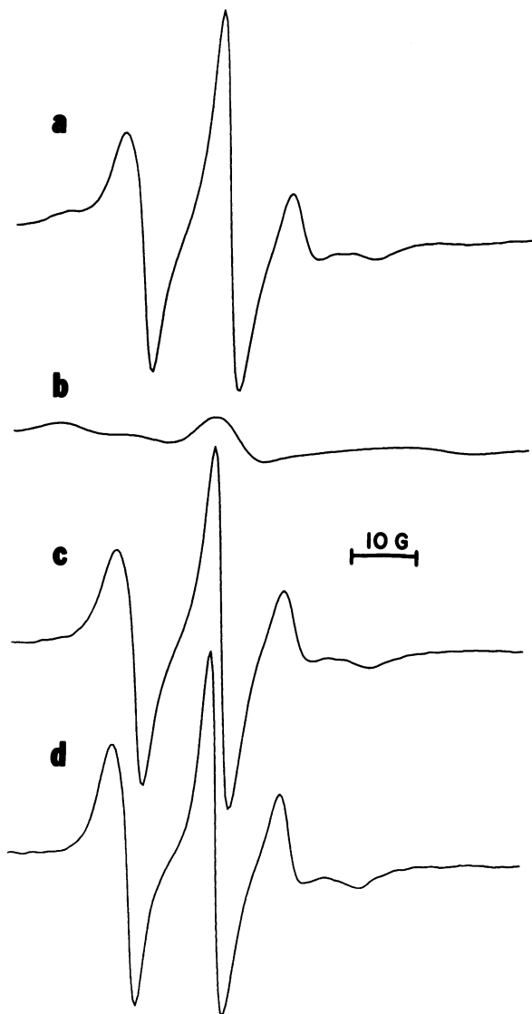
FIGURE 1 (a) EPR spectrum of 16-doxylstearic acid in AChR membranes prepared by a method similar to that of Elliott et al. (5) including base extraction. The \alpha -bungarotoxin binding activity was 2,000 pmol/mg protein. The lipid-to-spin probe ratio was 150:1. Incorporation of label was achieved by drying down the spin label in a glass tube and adding membranes. The membranes were pelleted and drawn into a 50 ml capillary tube for spectroscopy. (b) EPR spectrum simulated with the Nicolet EPRCAL program. g and a values were taken from (6). The correlation time was adjusted to give an outer splitting of 62.5 G. (c) Spectrum after subtraction. (d) Spectrum of 16-doxylstearic acid in liposomes prepared from Torpedo membrane lipids.
