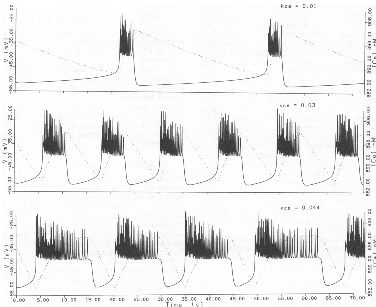
FIGURE 1 The burst behavior in response to increasing k_{Ca} , the Ca, efflux rate constant. The solid line shows the membrane potential, and the dashed line shows the associated changes in the concentration of intracellular Ca^{2+} ions. Here, the values of k_{Ca} 's used for the computation are, from the top panel to the bottom, 0.01 \text{ ms}^{-1} , 0.03 \text{ ms}^{-1} , and 0.044 \text{ ms}^{-1} , respectively.
