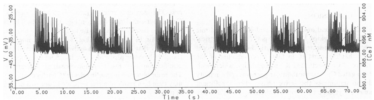
FIGURE 6 This figure compares the bursting behaviors with those shown in the top panel of Fig. 3 when g_x 's are doubled by a factor of two. Also, k_{Ca} was doubled, and f and \lambda (i.e., 0.68) were halved.
