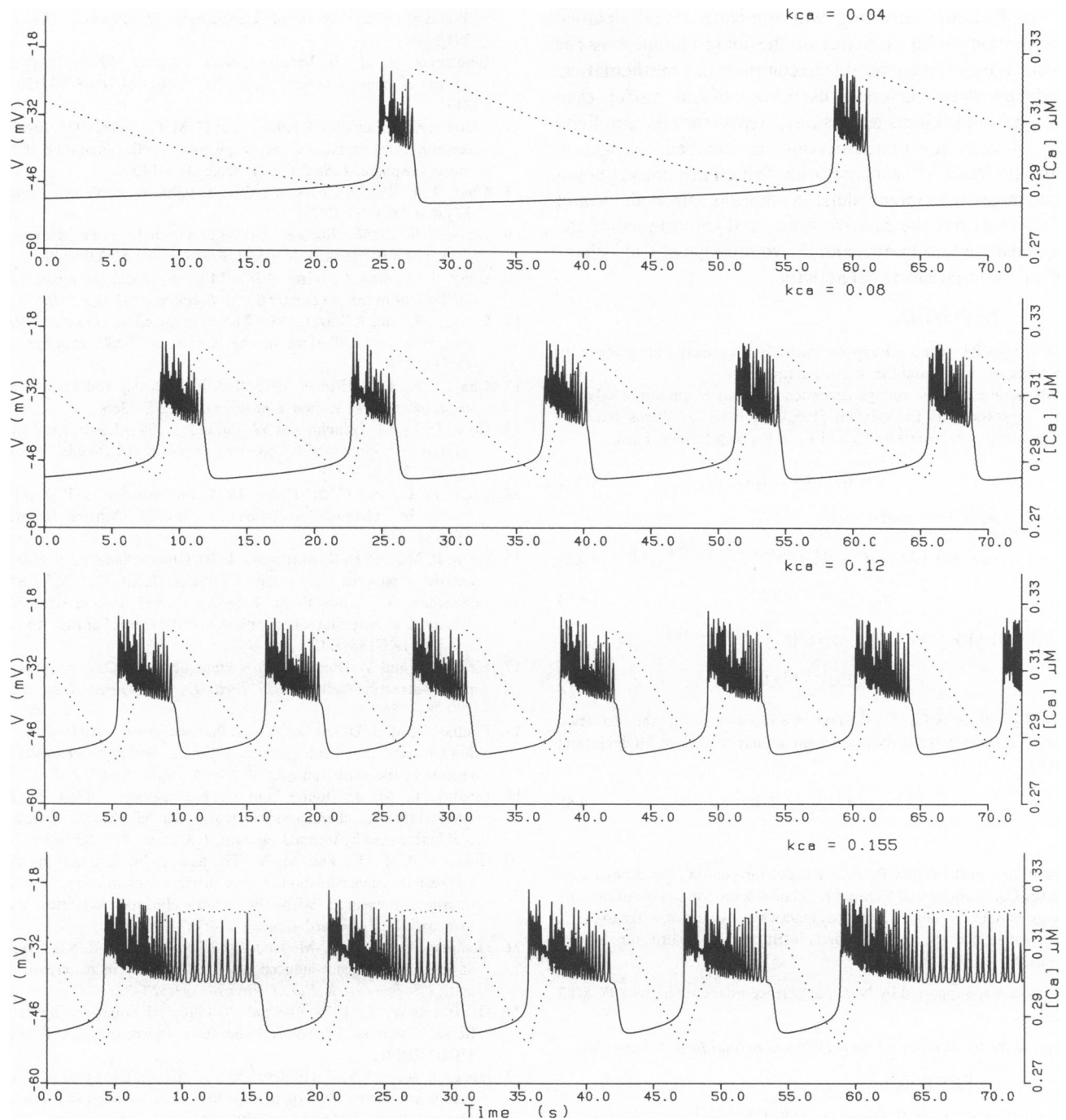
FIGURE 7 The burst behavior obtained by adding the inactivation term h_{\infty}^{0.3} to Eq. 5. Here, the values of k_{Ca} 's used for the computation are, from the top panel to the bottom, 0.04 \text{ ms}^{-1} , 0.08 \text{ ms}^{-1} , 0.12 \text{ ms}^{-1} , and 0.155 \text{ ms}^{-1} , respectively. Those parametric values that are different from Appendix B are: \bar{g}_{Ca} = 900 \text{ pS} , \bar{g}_{K,Ca} = 1,300 \text{ pS} , g_L = 20 \text{ pS} , V_n = -37 \text{ mV} , V_m = -50 \text{ mV} , A = -5 \text{ mV} , \lambda^{-1} = 1.3 , and f = 2 \times 10^{-4} .
