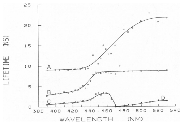
FIGURE 3 The decay times obtained by empirical deconvolution are shown as a function of wavelength, for 2,6 p -TNS adsorbed to L - \alpha -egg lecithin vesicles at the conditions described in the legend to Fig. 2. Curves A–D connect the decay times of the exponential terms from the empirical deconvolution in order to help demonstrate their continuously varying nature. Open squares represent decay times having a positive pre-exponent and closed squares represent decay times having a negative pre-exponent.
