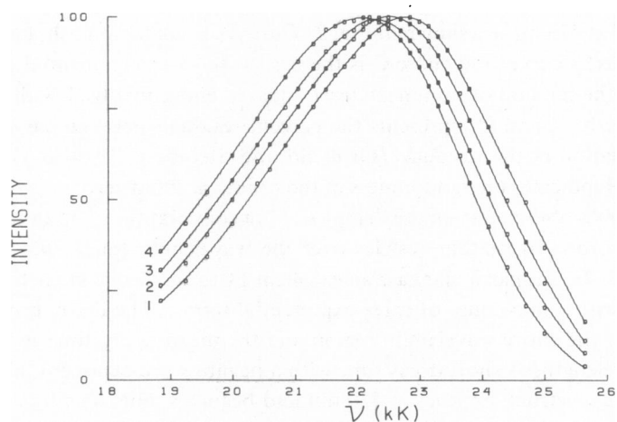
FIGURE 5 Peak normalized time-resolved emission spectra of 2,6 p -TNS adsorbed to L- \alpha -egg lecithin vesicles at the conditions described in the legend to Fig. 2. 1, 1.02 ns; 2, 2.04 ns; 3, 4.08 ns; 4, 12.24 ns. Spectra are corrected for instrumental wavelength response. Kilo-kayser (kK) = 10^3 \text{ cm}^{-1} .
