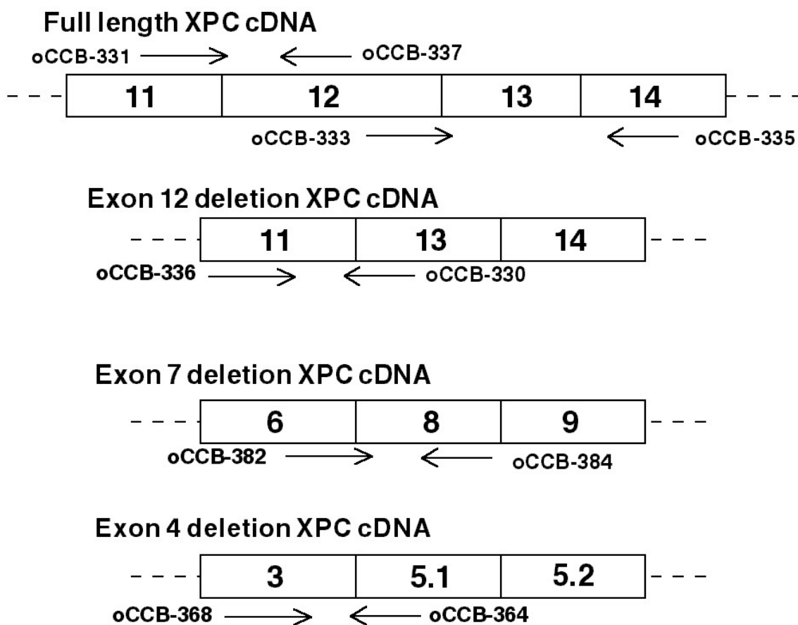
Figure S1. Primers used for real time quantitative reverse transcription polymerase chain reaction assays for XPC mRNA. A primer spanning the junction of adjacent exons was paired with a primer contained within another exon. Primer pairs were developed to measure full length XPC cDNA (including exon 12), deleting exon 12, deleting exon 7 or deleting exon 4.
