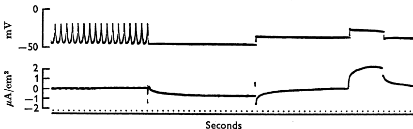
Fig. 1. Membrane currents recorded during step potential changes in voltage range of oscillation. The preparation was oscillating spontaneously and was initially clamped at the maximum negative potential ( -46 mV) reached during oscillation. The membrane was then depolarized to -36 and -25 mV, followed by repolarization to -36 mV. Owing to the current-limiting properties of the current micro-electrode the potential is not quite constant following depolarization to -25 mV. Note slow current changes activated by depolarizations and deactivated by hyperpolarizations.
