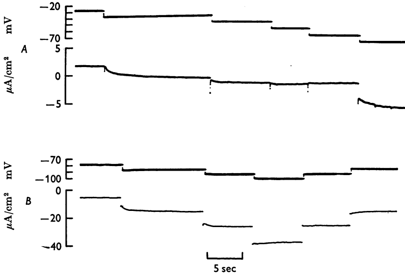
Fig. 3. Membrane current in response to 'staircase' hyperpolarization of the membrane from -27 to -100 mV. Step changes to -37 and -47 mV produce substantial slow current changes. At -57 and -67 mV there are virtually no slow current changes. On hyperpolarizing to -77 mV another large current change occurs. The responses to larger hyperpolarizations ( -85 , -93 and -100 mV) are shown on smaller amplification. Same preparation as in Fig. 1.
