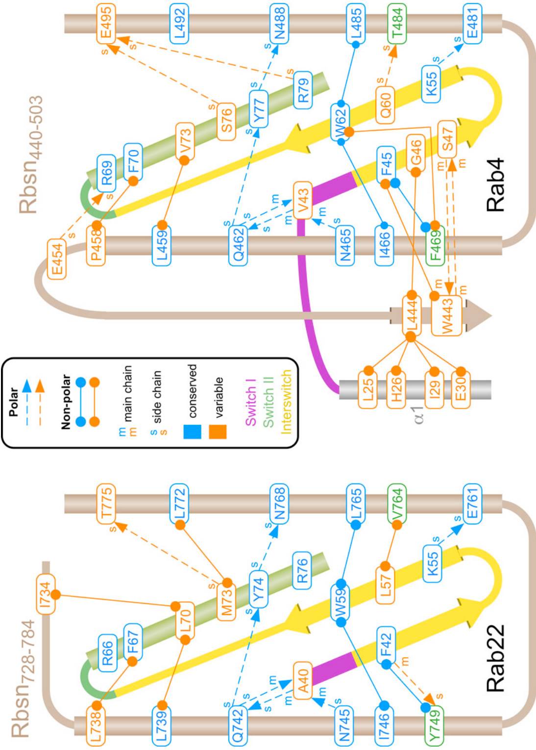
Supplementary Figure 6. Schematic diagram of intermolecular interactions in the Rab22-Rbsn 728-784 complex (left) and Rab4-Rbsn 440-503 complex (right).
