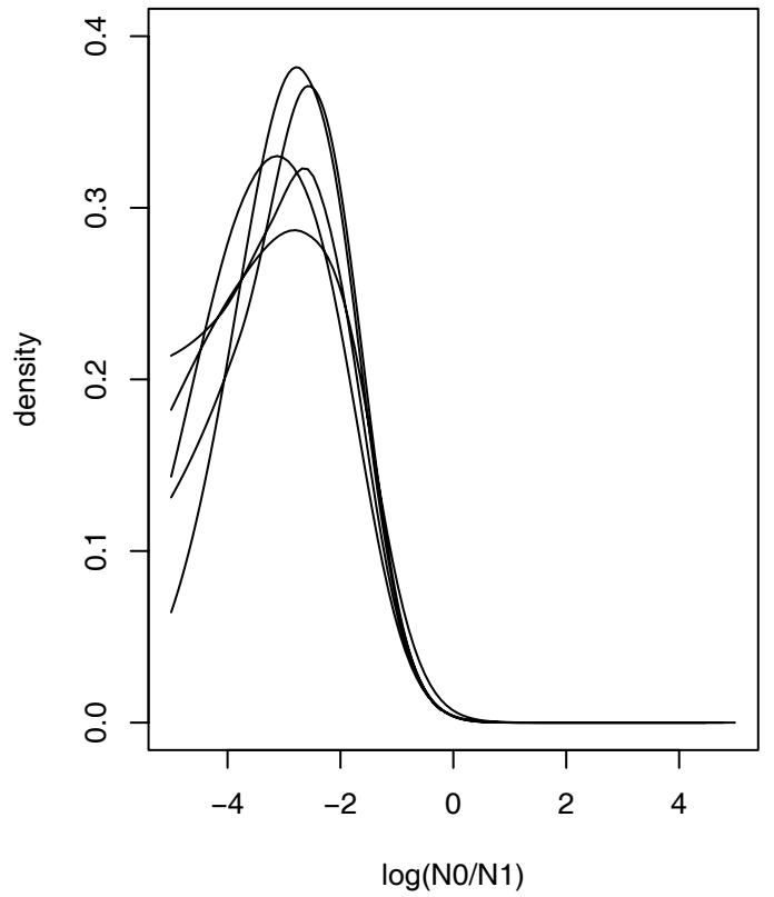
MCMC runs – exponential model (S1)
