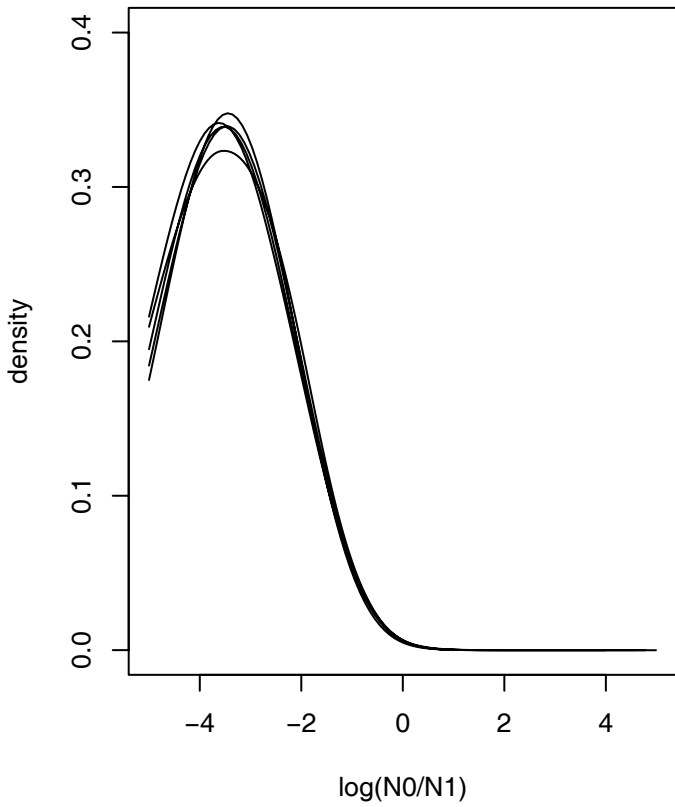
MCMC runs – linear model (S2)
