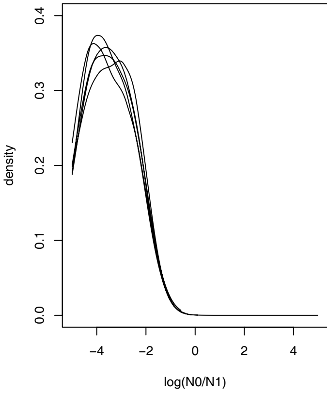
MCMC runs – linear model (S1)
