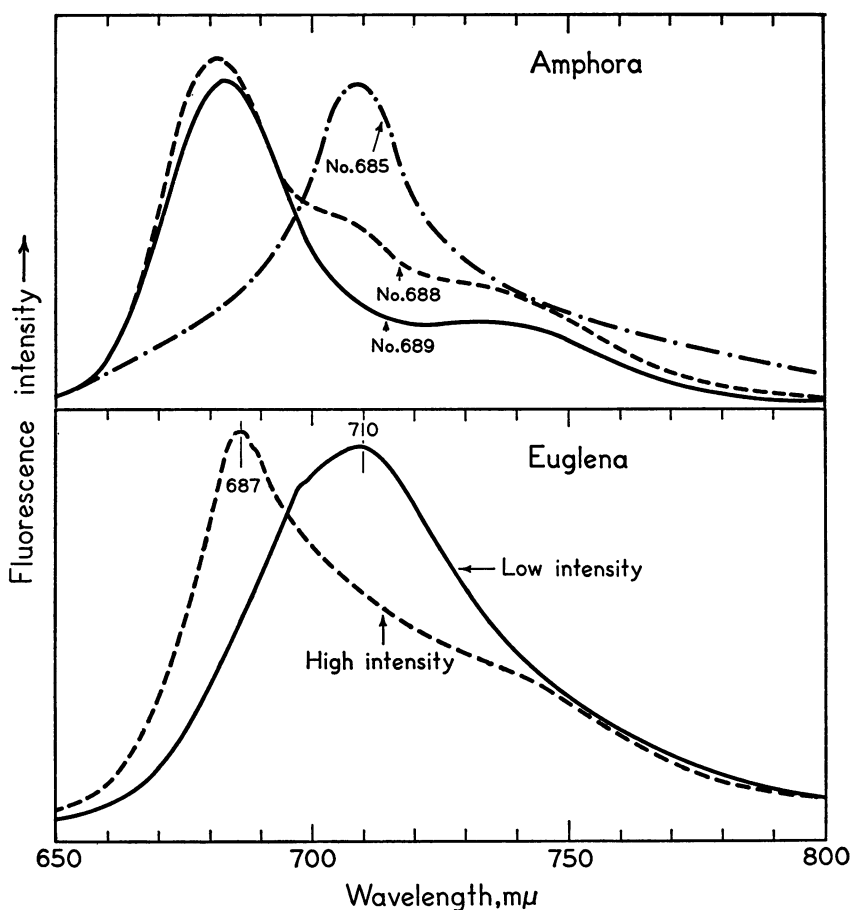
FIGURE 2 Fluorescence spectra of plants grown with different light intensities and containing various amounts of C_{695} . The fluorescence peak of C_{695} lies at 705 to 708 \mu . The Amphora cultures were from the Starr collection and are identified by Starr's number.
