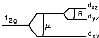
FIGURE 1 Crystal field parameters in terms of single orbital energy intervals.
