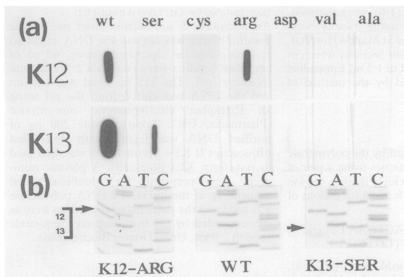
Slot-blot and sequence analysis of polymerase chain reaction amplified DNA extracted from a single colorectal adenoma for activating mutations of codons 12 and 13 of the human K-ras gene. (a) The autoradiographs of the filters show that the filters hybridised with codons 12 and 13 wild type specific probes (GGT-GLY and GGC-GLY, respectively). In addition, two of the mutant specific probes gave detectable signals: CGT-ARG at codon 12 and AGC-SER at codon 13. (b) Sequencing autoradiograms of the antisense strands of three clones show the existence of the three alleles inferred from (a) above: mutant at codon 12 (ACG'-ARG); wild type at codons 12 (ACC'-GLY) and 13 (GCC'-GLY); and mutant at codon 13 (GCT'-SER). Arrows denote mutant bases.
