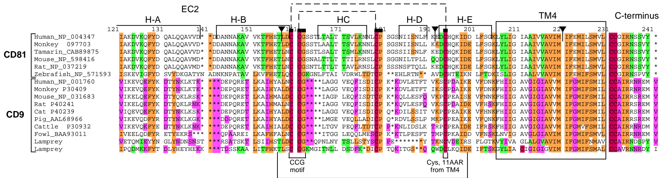
Region involved in association with diphtheria toxin receptor (DTR)
