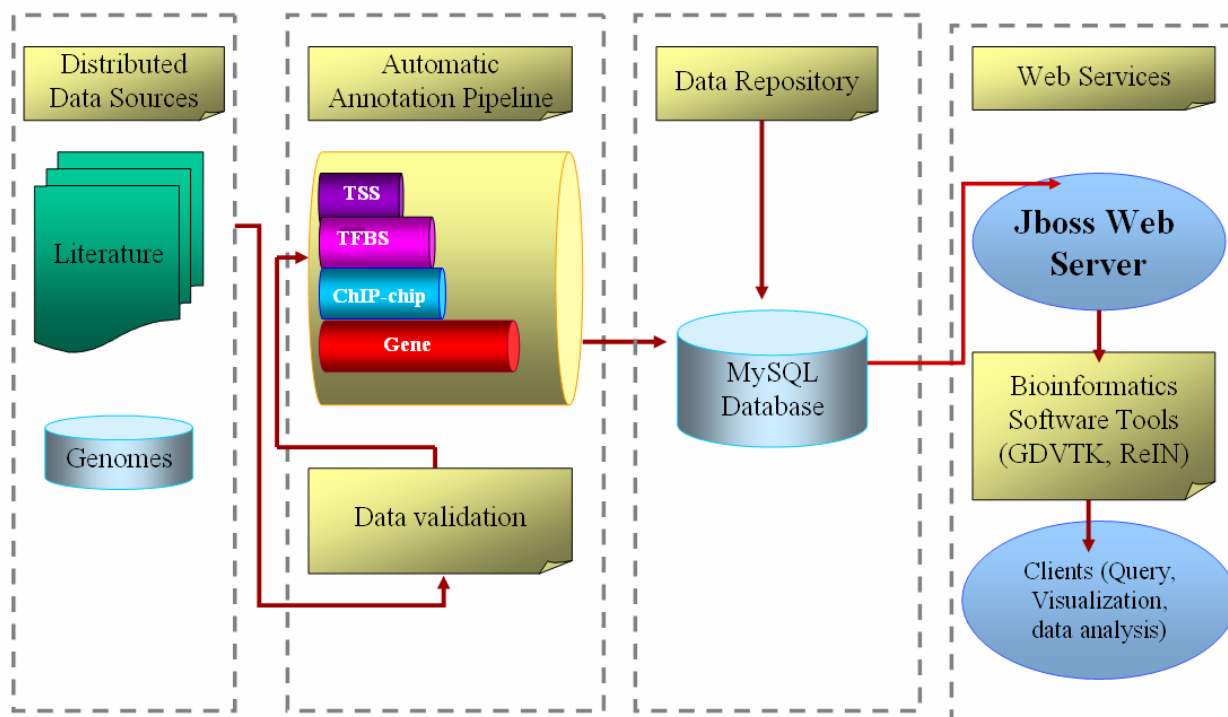
Supplemental Figure 1. Schematic overview of Bioinformatics Infrastructure describing data access and its web interface architecture
