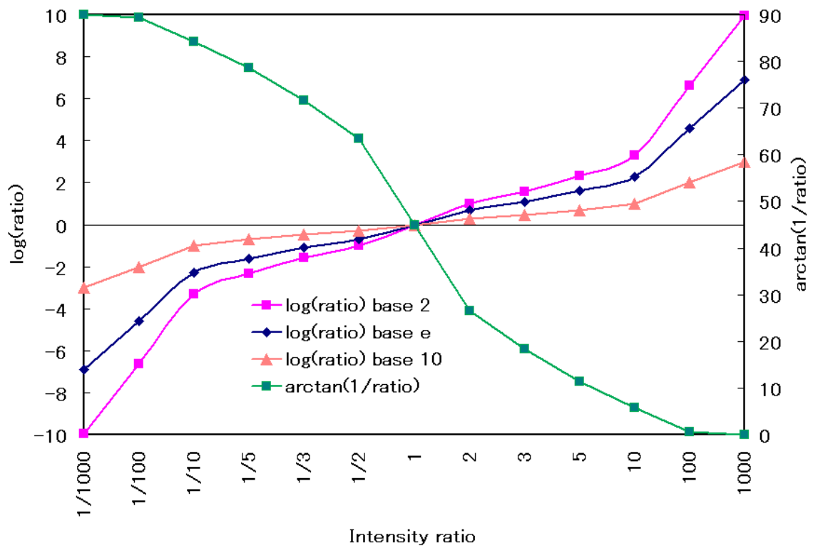
Supplementary Figure 1 A new index [ \arctan(1/\text{ratio}) ] and current log transformed indices [ \log(\text{ratio}) ] for gene expression ratios.
