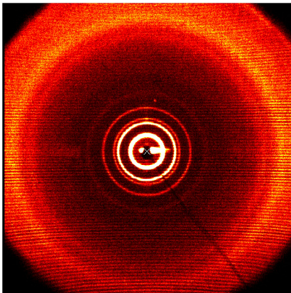
(4-3,4-3,5) 4G2CH 2 OH 25°C (as prepared, 1 st heating)
