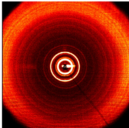
(4-3,4-3,5) 4G2CH 2 OH 85°C (1 st cooling)
