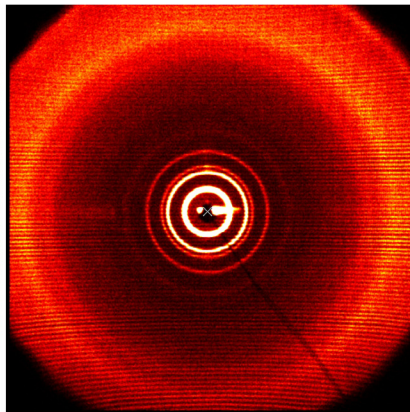
(4-3,4-3,5) 4G2CH 2 OH 90°C (as prepared, 1 st heating)
