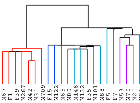
Supplementary figure S1 226 "intrinsic" gene cluster diagram
