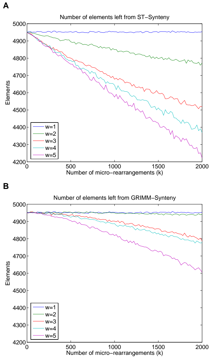
Figure S2. Number of elements retained in simulations after deletion of small blocks. Number of elements retained by (A) ST-Synteny and (B) GRIMM-Synteny, as a function of the number of micro-rearrangements k and micro-rearrangement size w in the simulated data.
