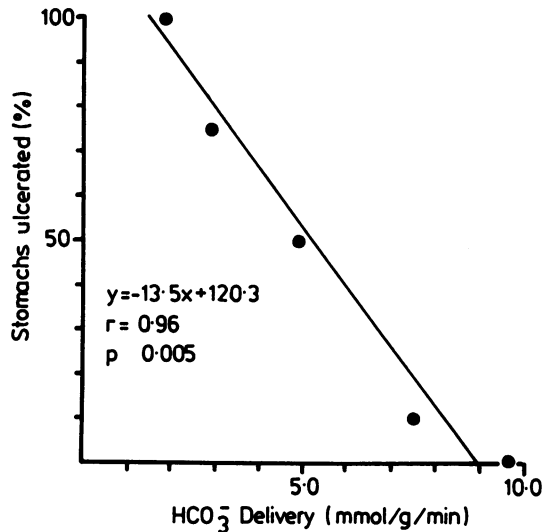
Fig. 2 Dependence of gastric mucosal damage (expressed as per cent of stomachs ulcerated) on \text{HCO}_3^- delivery by blood flow (mucosal blood flow determined with radioactive microspheres) in stomachs of rats subjected to haemorrhagic shock with and without infusion of \text{PGI}_2 and \text{HCO}_3^- (points represent means of each experimental group, ref 2).
