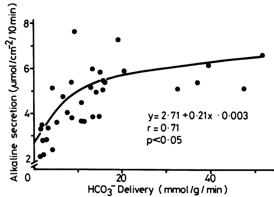
Fig. 1 Correlation of alkaline secretion and \text{HCO}_3^- delivery in rabbit duodenum. Mucosal blood flow determined with radioactive microspheres. Alteration of blood flow and arterial \text{HCO}_3^- concentration with iv infusion of vasopressin, \text{HCO}_3^- and \text{NH}_4\text{Cl} .
