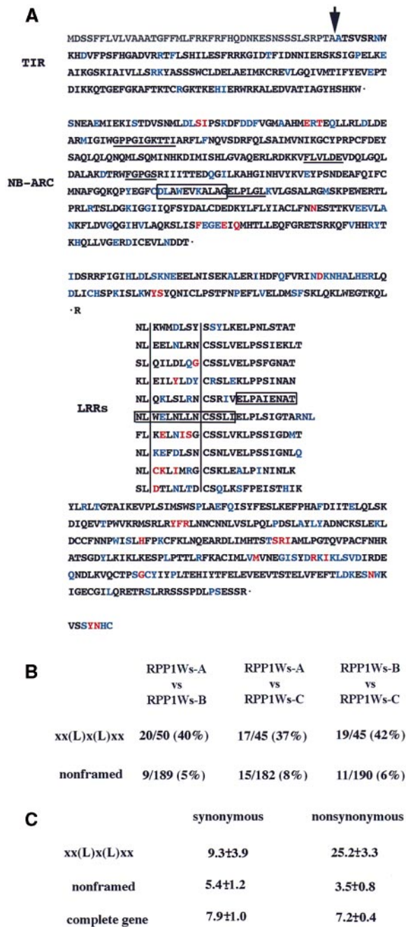
Figure 6. Structural Domains of the RPP1 Protein Family and Analysis of Their LRRs.
