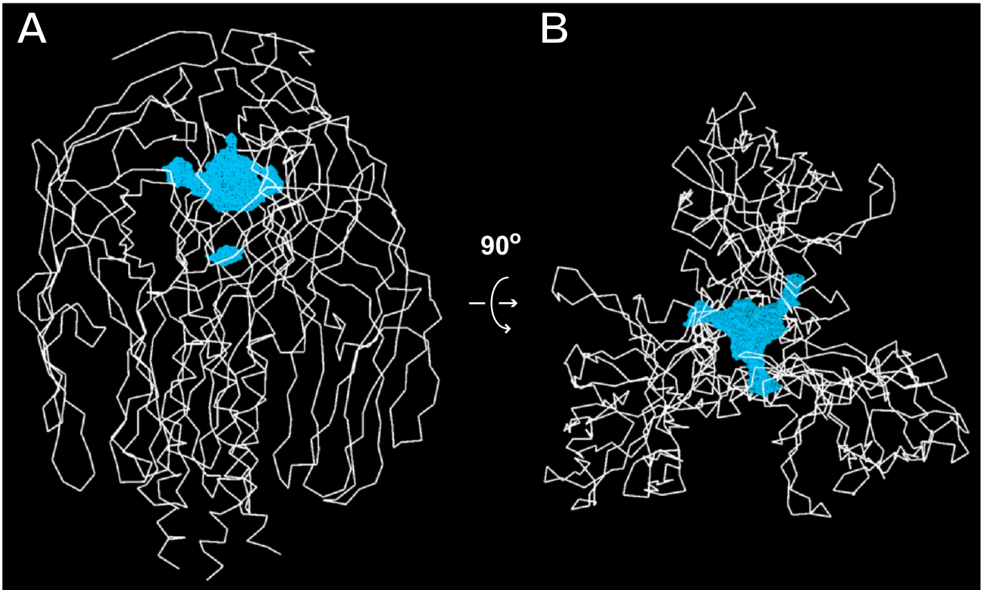
Internal cavities of VP5CT. Mesh models (cyan) of the internal cavities are shown within line drawings (white) of the VP5CT C \alpha trace. The mesh models show the volume accessible to a probe with a 1.4 Å radius, reflecting the volume potentially accessible to solvent. (A) Viewed from the side. (B) Viewed from the top.
