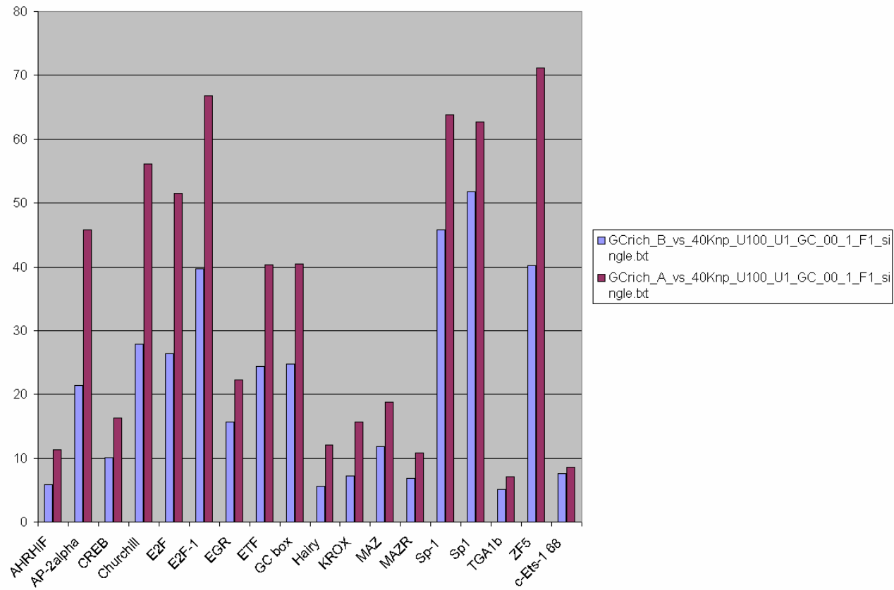
Figure S2. Distributions of TFs found to be common among the top 150 PEs in comparisons of different TSS types
