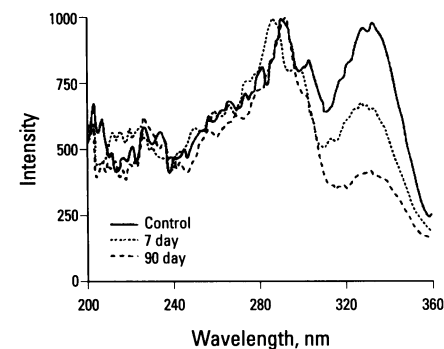
Figure 1. Representative excitation scan of an NMBA-induced esophageal carcinogenesis model within Sprague-Dawley rats. Rats were exposed to saline (control) or NMBA for 7 and 90 days, respectively. Fluorescence analysis reveals progressive loss of intensity of the 330-nm peak relative to the 290-nm peak with continued exposure. Reprinted from Glasgold et al. (24), with permission.
