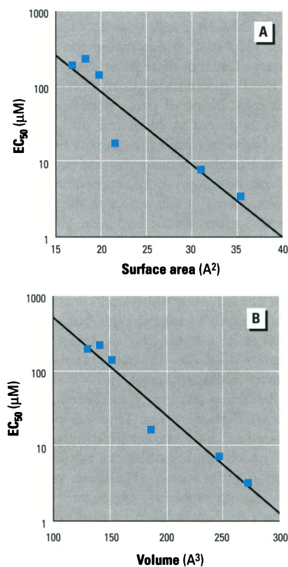
Figure 3. Correlation between P-gp inhibition potency and molecular surface area (A) or volume (B) of the pesticides. Potency is described by the effective concentration ( EC_{50} ) values as previously determined (12). Molecular surface area and volume of the pesticides are presented in Table 2.
