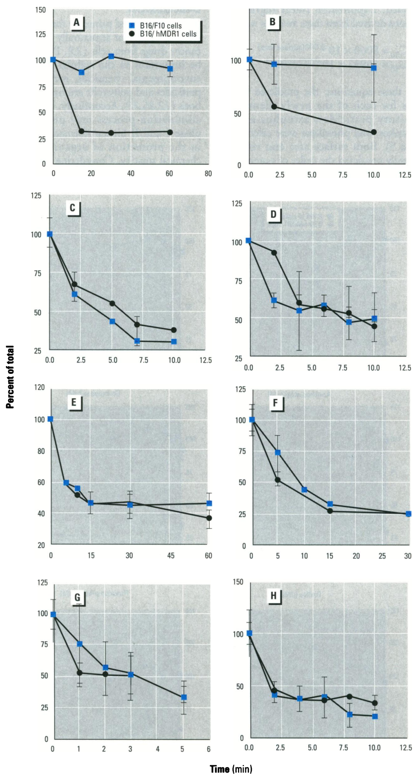
Figure 1. Efflux of pesticides from B16 cells. B16/F10 cells and B16/hMDR1 cells were incubated in (A) 50 \mu\text{M} doxorubicin; (B) 7 \mu\text{M} vincristine; (C) 100 \mu\text{M} phosalone; (D) 100 \mu\text{M} dialifos; (E) 100 \mu\text{M} azinphos-ethyl; (F) 100 \mu\text{M} coumaphos; (G) 100 \mu\text{M} fluzafop p -butyl; and (H) 100 \mu\text{M} triforine for 4 hr and allowed to deplete the accumulated pesticide (as described in Materials and Methods). The amount of pesticide remaining in the cells was analyzed by HPLC and is presented as percentage of the initial concentration of pesticide in the cells at the start of the depuration phase. Values are the mean \pm standard deviation of three replicates for each time point.
