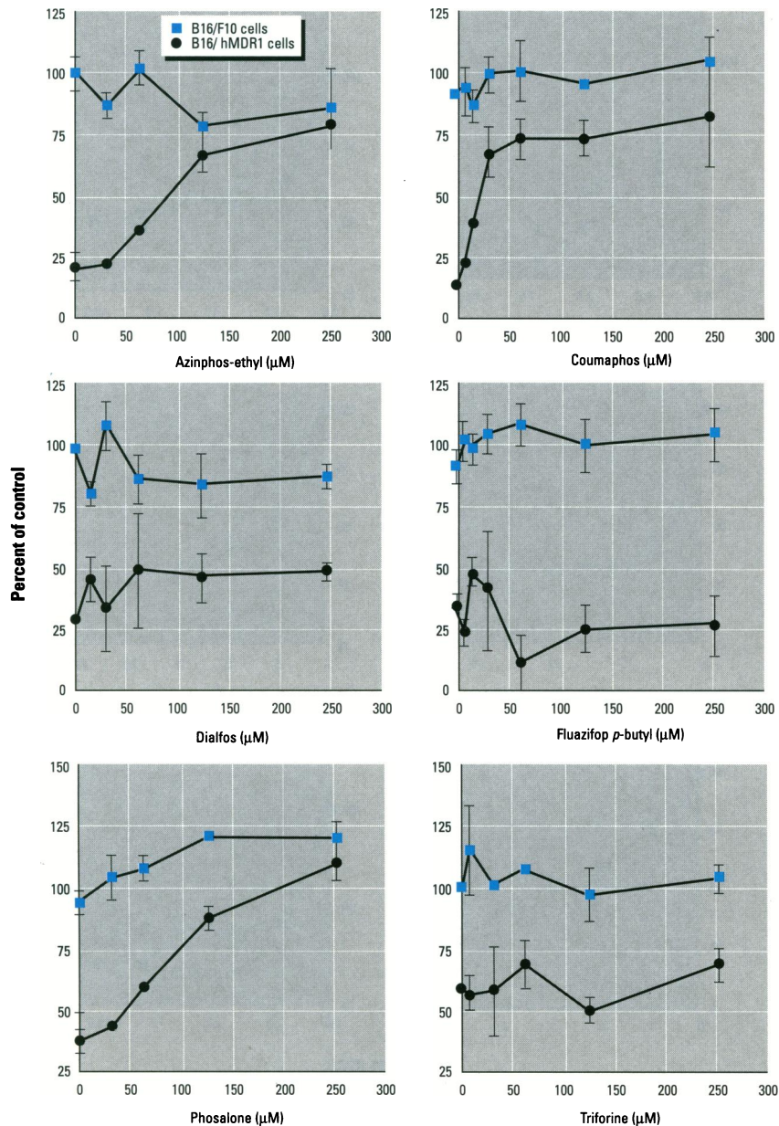
Figure 2. Inhibition of P-gp-mediated doxorubicin efflux by pesticides. B16/F10 cells and B16/hMDR1 cells were incubated for 4 hr in 50 \mu\text{M} doxorubicin along with increasing concentrations of the pesticides. The amount of doxorubicin accumulated in the cells was measured fluorimetrically and is presented as the percentage of the amount of doxorubicin measured in the positive control cells incubated in 10 \mu\text{M} verapamil. Values are the mean \pm standard deviation of three replicates for each concentration of pesticide.
