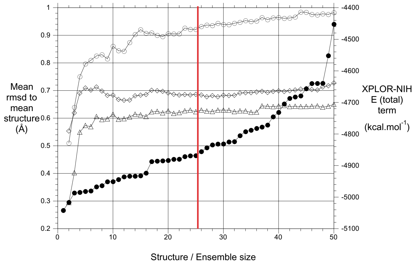
Supplementary figure 5. Energy-ordered rmsd profiles and total energies for the 50 calculated structures of Hrp1-PEE complex. Filled black circles represent the total XPLOR Energy values (scale on the right vertical axis). Rmsd values were calculated for the overall structure (residues 160-318; open circles) and separately for the RBD1 (160-234; diamonds) and RBD2 (234-318; up triangles) domains (scale on the left vertical axis). The red line represents the chosen cut-off for the final ensemble of structures (Table 1).
