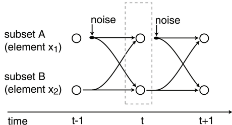
(b) outputs from A are replaced by noise
