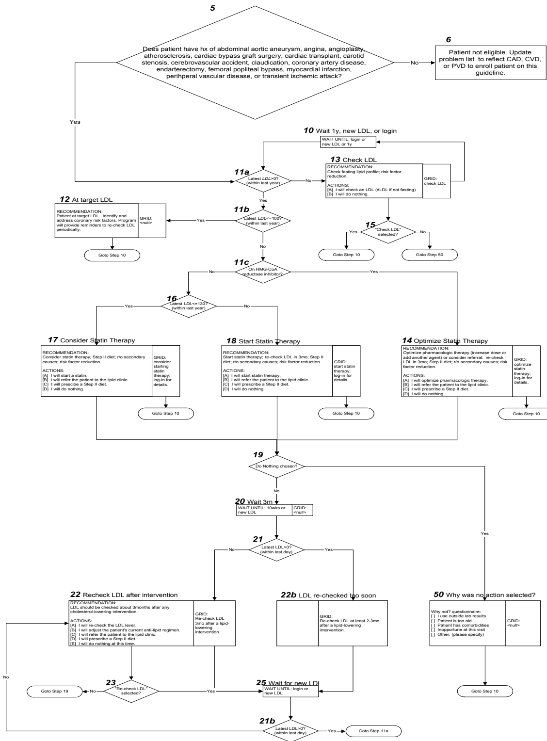
Figure 3. Flowchart (Visio®) specification of the NCEP secondary prevention guidelines, adapted from the published guidelines with local experts, and then entered into P-CAPE. Diamonds represent Decision steps, and rectangles Action steps. The ovals are re-directors that are actually defined within Action steps, but separated out here for clarity.
