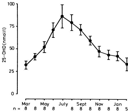
FIG 2—Mean ± SEM serum 25-OHD concentrations in eight normal subjects throughout year.
