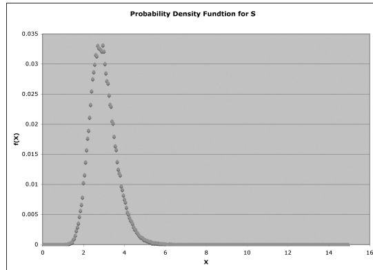
Supplementary Figure 2: Distribution of S for sample size 6: Probability Density Function
