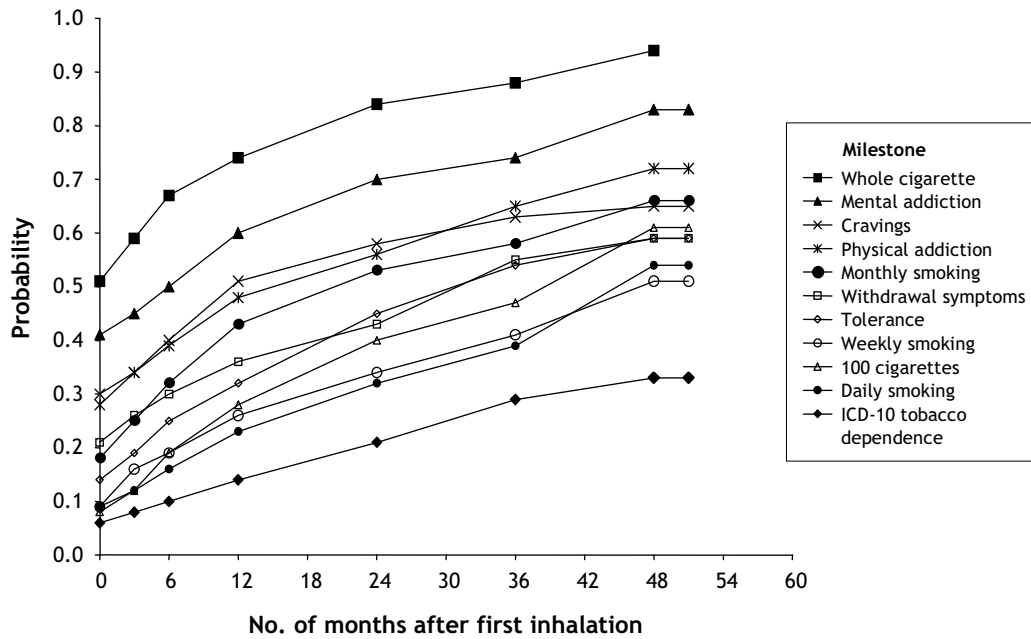
Appendix 3: Cumulative probability of attaining each milestone of smoking onset in subgroup of participants who reported inhaling into lungs ( n = 253 ), according to number of months after first inhalation. (See Methods of main article for definitions of milestones [available at www.cmaj.ca/cgi/content/full/175/3/255 ].)
