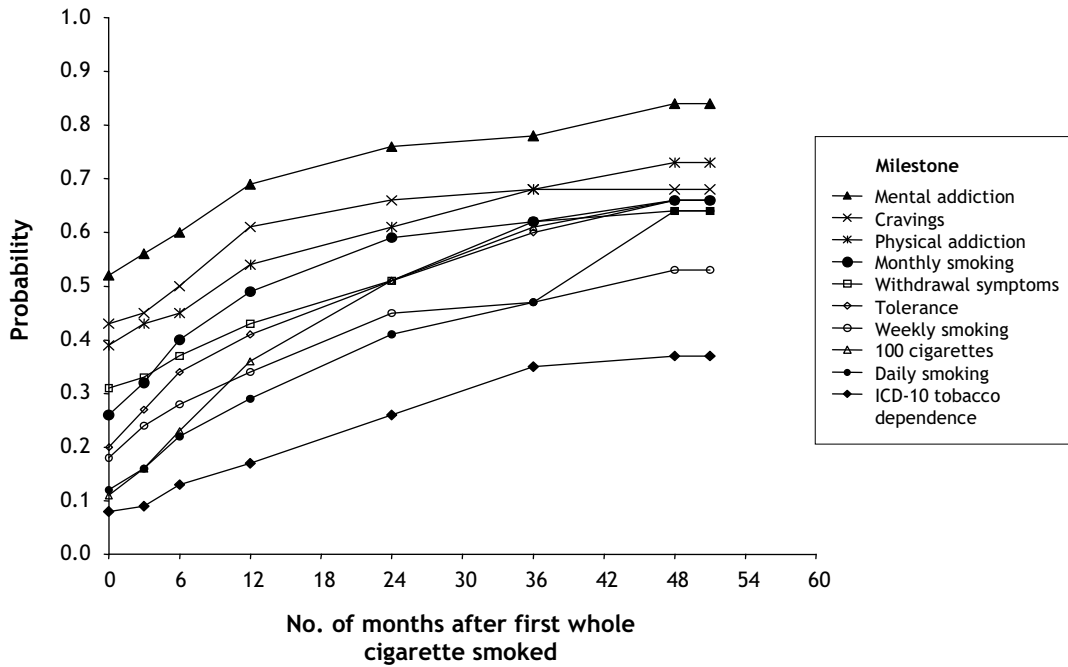
Appendix 4: Cumulative probability of attaining each milestone of smoking onset in subgroup of participants who reported smoking a whole cigarette ( n = 214 ), according to number of months after first whole cigarette smoked. (See Methods of main article for definitions of milestones [available at www.cmaj.ca/cgi/content/full/175/3/255 ].)
