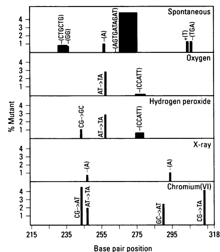
Figure 10. Kinds, positions, and frequencies of 6TG mutations induced by K_2Cr_2O_7 , O_2 , H_2O_2 , X-rays in the low melting domain of exon 3 on the hprt gene in human lymphoblastoid B-cells (TK6) (10).
