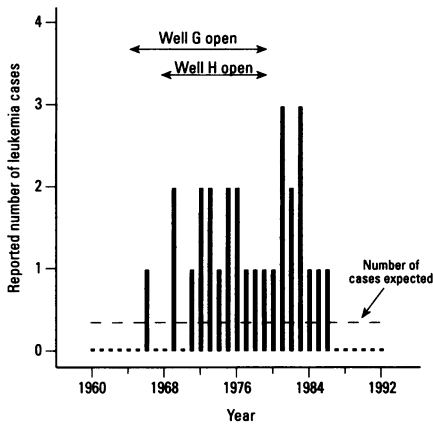
Figure 2. Incidence of childhood leukemia cases in Woburn, Massachusetts, between 1960 and 1992. The expected number of cases in Woburn (population approximately 36,000) for persons 0 to 19 years of age was 0.3 per year (2).
