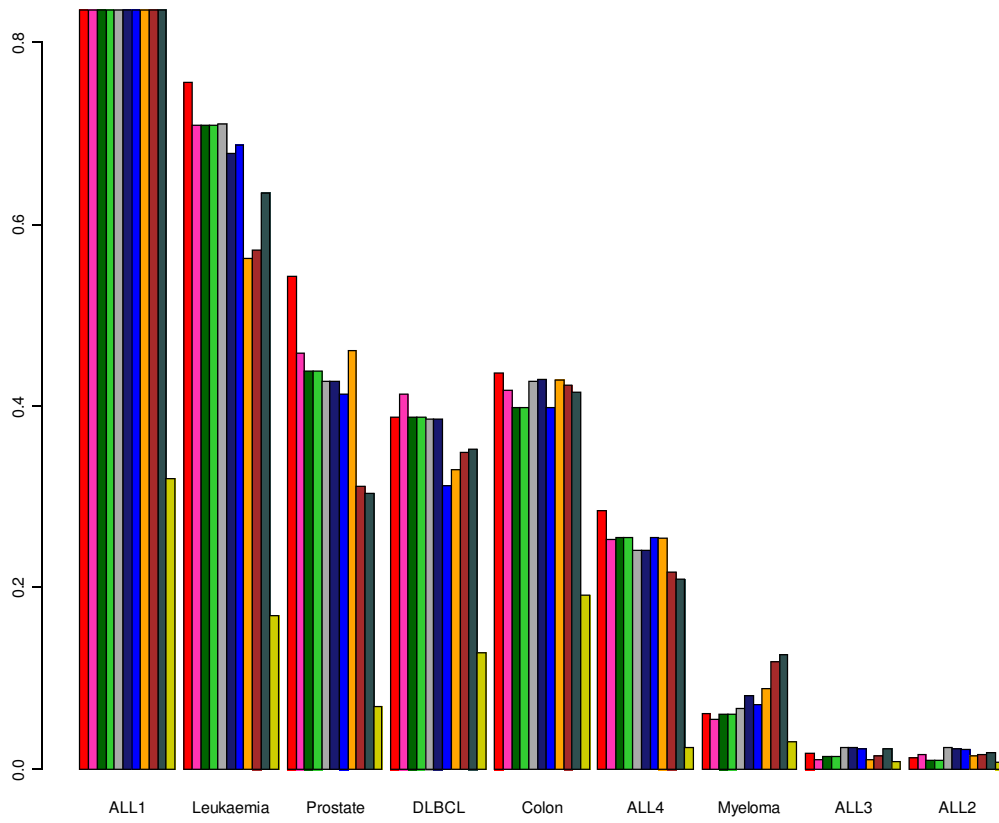
Split Sample. Training and Test. BGA classifier
